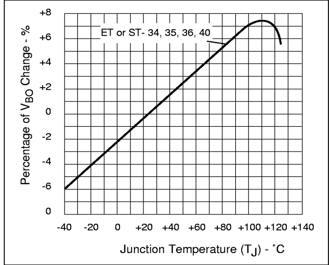
Figure 2: Normalized V_{BO} Change vs. Junction Temperature
