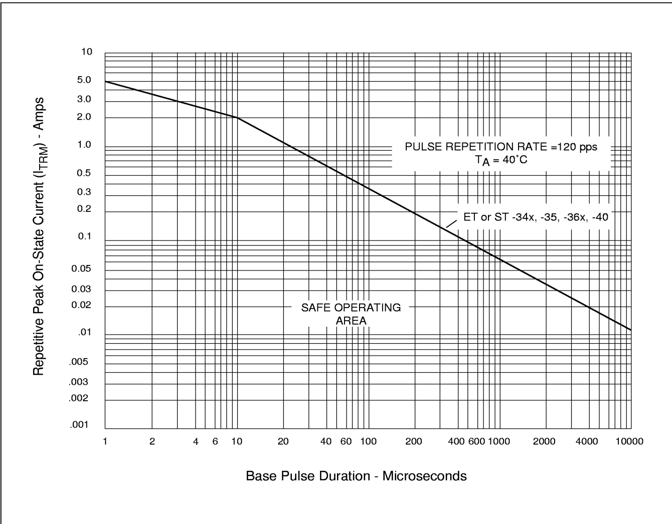
Figure 3: Repetitive Peak On-State Current vs. Pulse Duration
