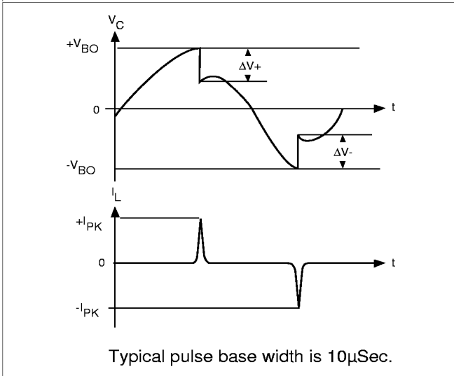
Figure 4: Test Circuit Waveforms (see figure 5).
