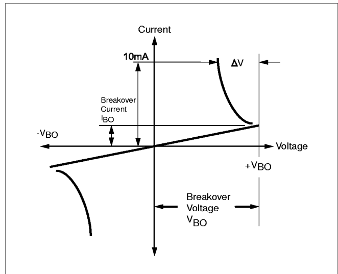
Figure 7: V-I Characteristics
