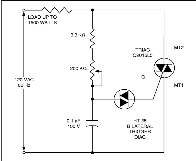
Figure 1: Typical Diac-Triac Full-Wave Phase Control Circuit using Lower Voltage Diacs.
