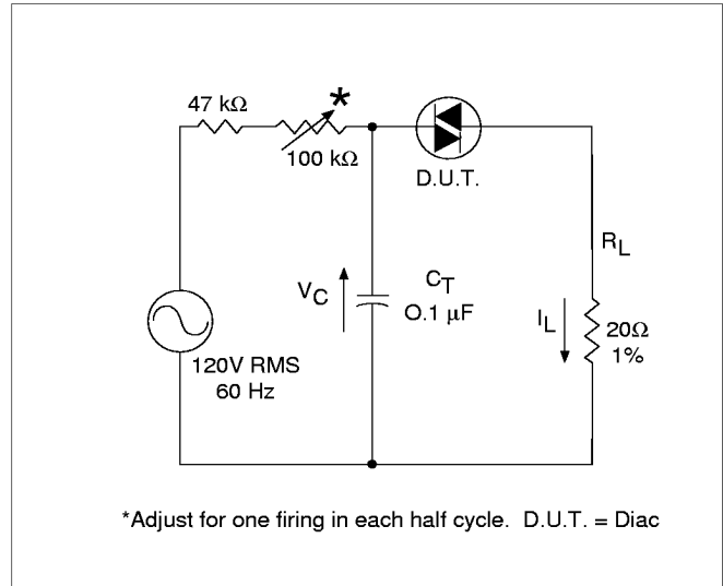
Figure 5: Circuit Used to Measure Diac Characteristics (See Figure 4.)
