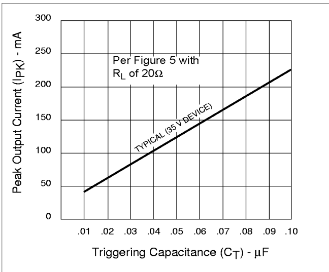
Figure 6: Peak output Current vs. Triggering Capacitance
