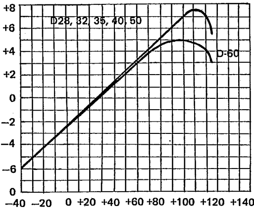
FIGURE 3- NORMALIZED VBO CHANGE VS JUNCTION TEMPERATURE
