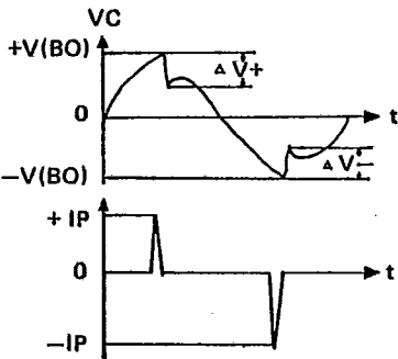
FIGURE 4- TEST CIRCUIT WAVEFORMS (SEE FIGURE 5)
