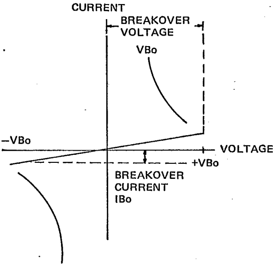
FIGURE 1- V-I CHARACTERISTICS
