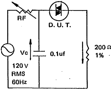
FIGURE 5- CIRCUIT USED TO MEASURE DIAC CHARACTERISTICS
