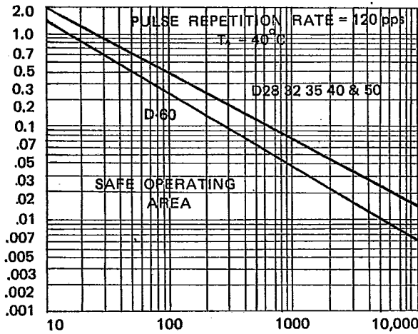
FIGURE 2- REPETITIVE PEAK ON-STATE CURRENT VS PULSE DURATION
