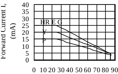
FIG.3 ALLOWABLE DC CURRENT VS. AMBIENT TEMPERATURE
