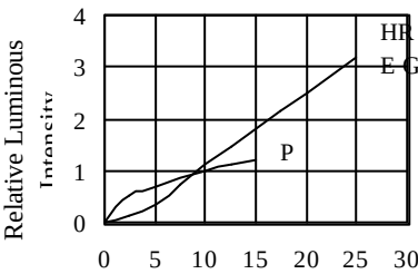
FIG.2 RELATIVE LUMINOUS INTENSITY VS. FORWARD CURRENT
