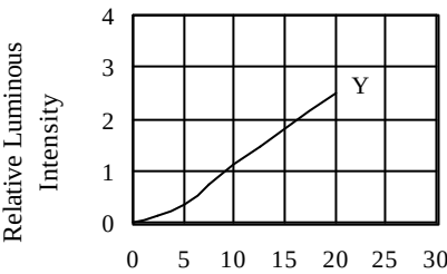
FIG.2-1 RELATIVE LUMINOUS INTENSITY VS. FORWARD CURRENT
