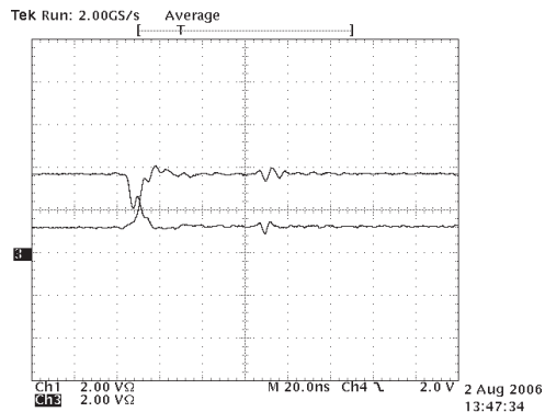
Driver Output Waveforms High to Low
