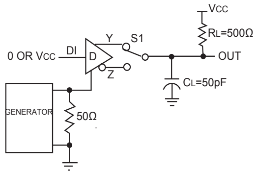
Driver Enable and Disable Times Test Circuit and Timing Diagram
