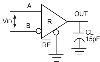
Receiver Propagation Delay Test Circuit and Timing Diagram
