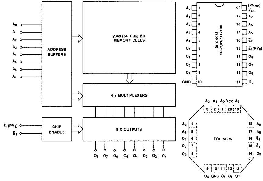
MB7117E/H, MB7118E/H Block Diagram and Pin Assignment
