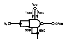
Both gates are tested simultaneously. FIGURE 6. I_{CCH} , I_{CCL}
