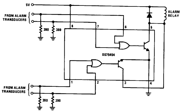
FIGURE 24. Alarm Detector
