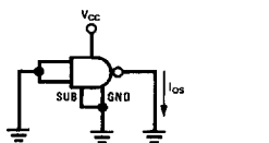
Each input is tested separately. FIGURE 5. I_{OS}
