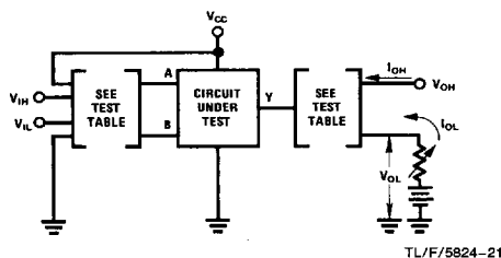
FIGURE 7. V_{IH} , V_{IL} , I_{OH} , V_{OL}
