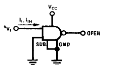
Each input is tested separately. FIGURE 4. I_I , I_{IH}
