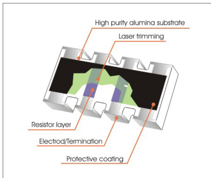
Fig 1. Constraction of a Chip-R array WA04
