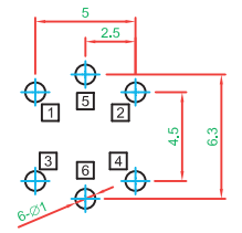
P.C.B. LAYOUT (Right Angle Type)
