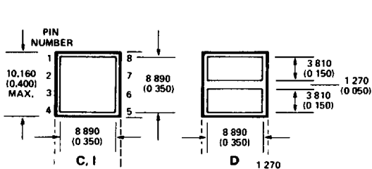
SIDE A
