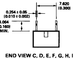
END VIEW C, D, E, F, G, H, I
