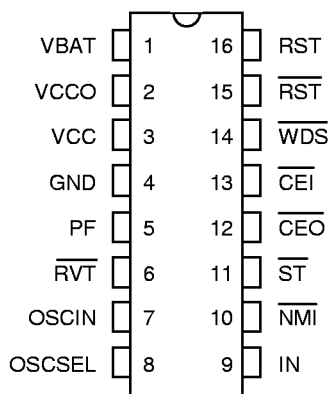
16-Pin DIP (300-mil) See Mech. Drawings Section
