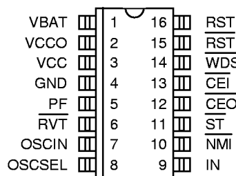
16-Pin SOIC (300-mil) See Mech. Drawings Section
