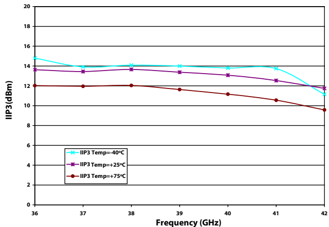
LSB IIP3 for XU1006-QB Vg2=-0.5V, Vd=4V, Id=240mA, P_LO=+4dBm, P_IF/1tone=-5dBm, ?F=10 MHz
