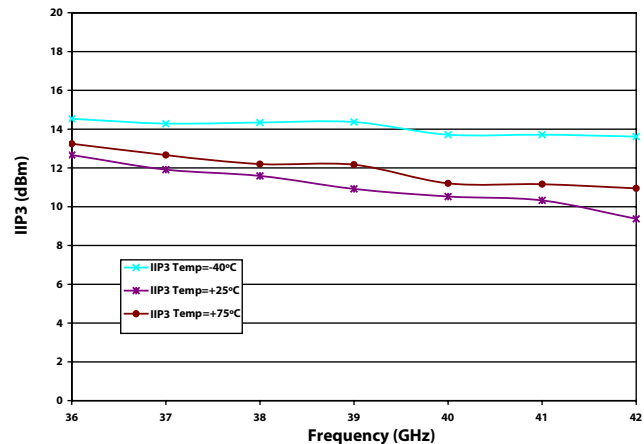
USB IIP3 for XU1006-QB Vg2=-0.5V, Vd=4V, Id=240mA, P_LO=+4dBm, P_IF/1tone=-5dBm, ?F=10 MHz
