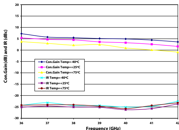
LSB Conversion Gain (dB) and IR (dBc) for XU1006-QB Vg2=-0.5V, Vd=4V, Id=240mA, P_LO=+4dBm, P_IF=-10dBm, IF_Frequency=2 GHz
