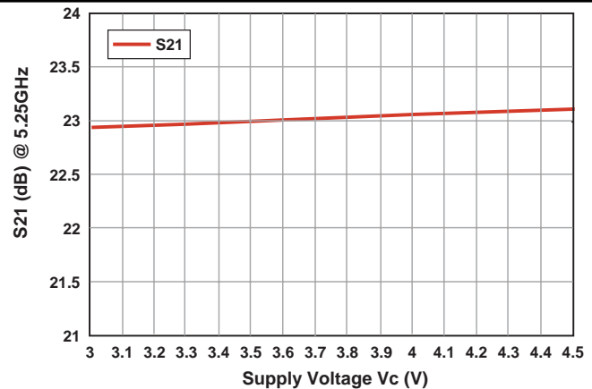
Typical Small Signal Gain vs. Supply Voltage (R_6 = 0\Omega, V_{ref} = 2.9V, I_{cq} = 100mA \text{ for } V_c = 3.3V, \text{Freq} = 5.25GHz)
