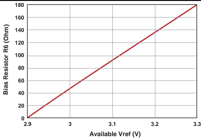
Recommended Bias Resistor for Available Vref (\text{Adjusted } R_6 \text{ value for Obtaining Nominal } I_{cq} = 10mA \text{ at } V_c = 3.3V)
