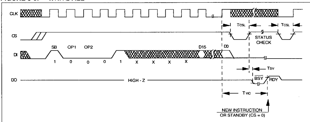
FIGURE 3-6: WRITE ALL
