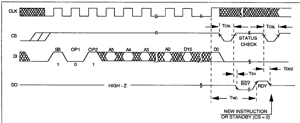
FIGURE 3-2: WRITE MODE
