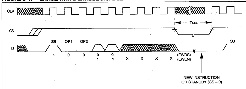
FIGURE 3-4: ERASE/WRITE ENABLE/DISABLE
