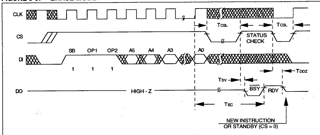
FIGURE 3-3: ERASE MODE
