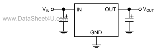
Figure 3. Linear regulators require only two capacitors for operation.
