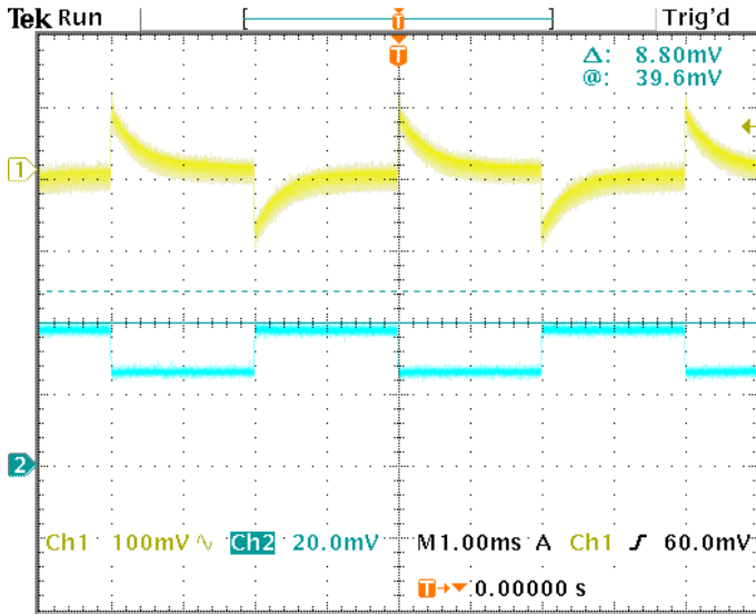
Fig 13. Dynamic response of load step at Vin=48v, Ch1: output voltage change(100mv/div), Ch2: output current step of 50%-75%-50% (2A/div). Current slew rate:0.1A/μs, Co=10μF tantalum capacitor + 1μF Ceramic capacitor, time scale: 1ms/div
