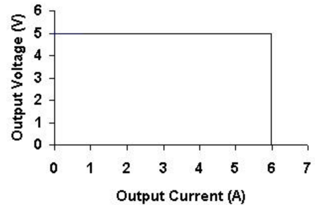
Fig 16. Output voltage vs current showing current limit point and converter shut down point
