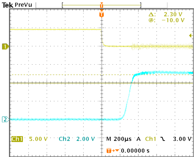
Fig 10. Startup under negative logic control at V_{in}=48v , I_{out}=5A . Ch1: ON/OFF signal (5V/div), Ch2: Output voltage (2V/div), C_o=10\mu F tantalum capacitor + 1\mu F Ceramic capacitor, time scale: 200 \mu s /div
