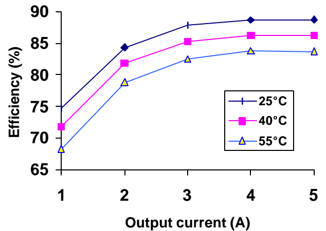
Fig 12. Efficiency at nominal input (48V) vs. load at different ambient temperatures of 25°C, 40°C, 55°C without air flow, the input voltage is 48V.
