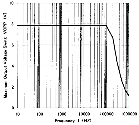
NJM14558 Maximum Output Voltage Swing vs. Frequency
