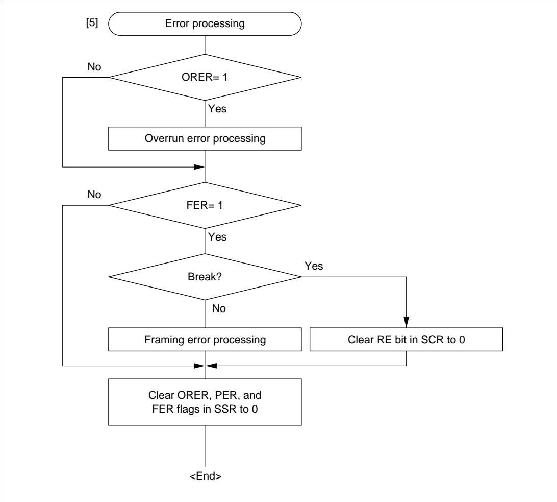
Figure 16-12 Sample Multiprocessor Serial Reception Flowchart (cont)
