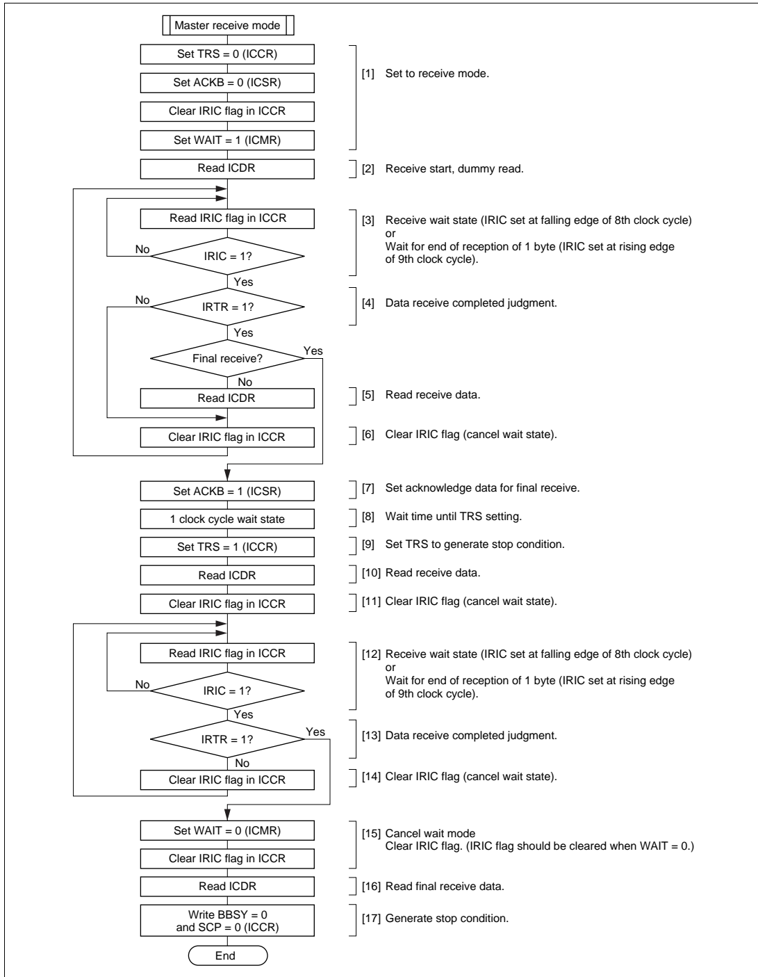
Figure 18-10 Flowchart for Master Receive Mode (Receiving Multiple Bytes) (WAIT = 1) (Example)
