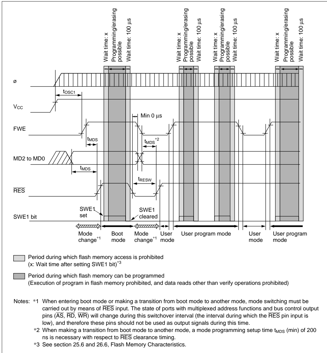
Figure 22-29 Mode Transition Timing (Example: Boot Mode \rightarrow User Mode \leftrightarrow User Program Mode)
