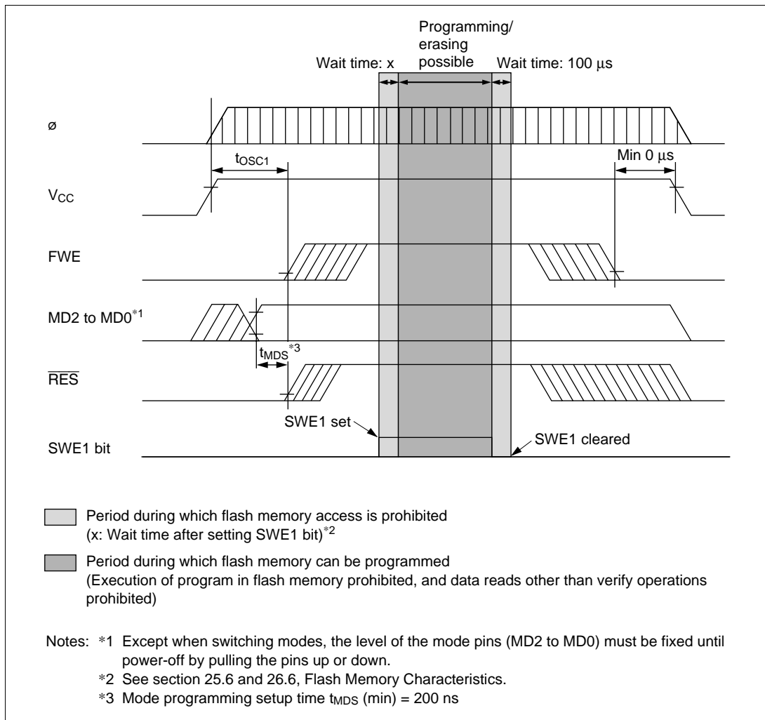
Figure 22-28 Power-On/Off Timing (User Program Mode)
