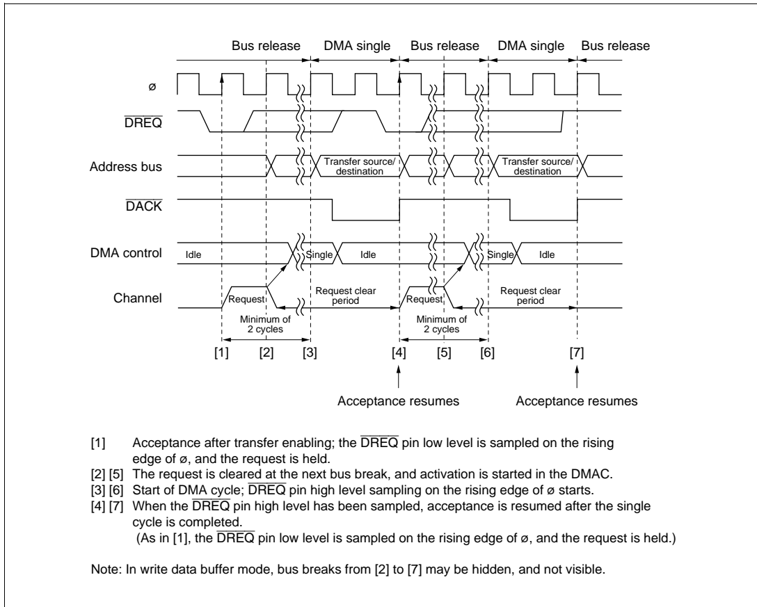
Figure 8-31 Example of \overline{\text{DREQ}} Pin Falling Edge Activated Single Address Mode Transfer
