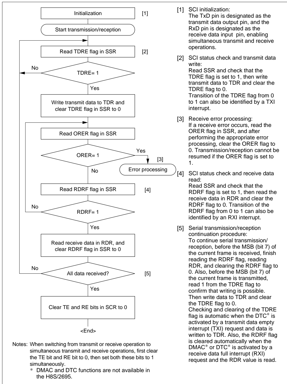
Figure 16-20 Sample Flowchart of Simultaneous Serial Transmit and Receive Operations
