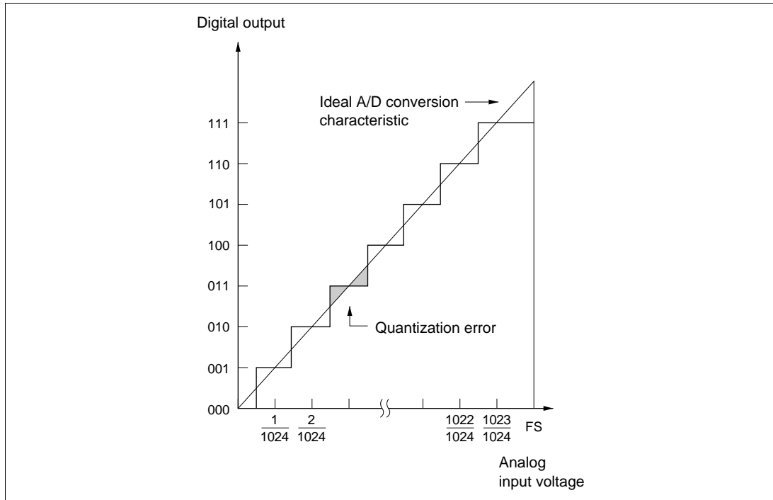
Figure 19-9 A/D Conversion Precision Definitions (1)
