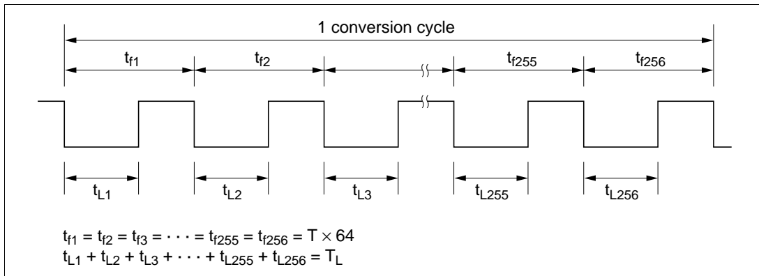
Figure 14-4 (1) Output Waveform
