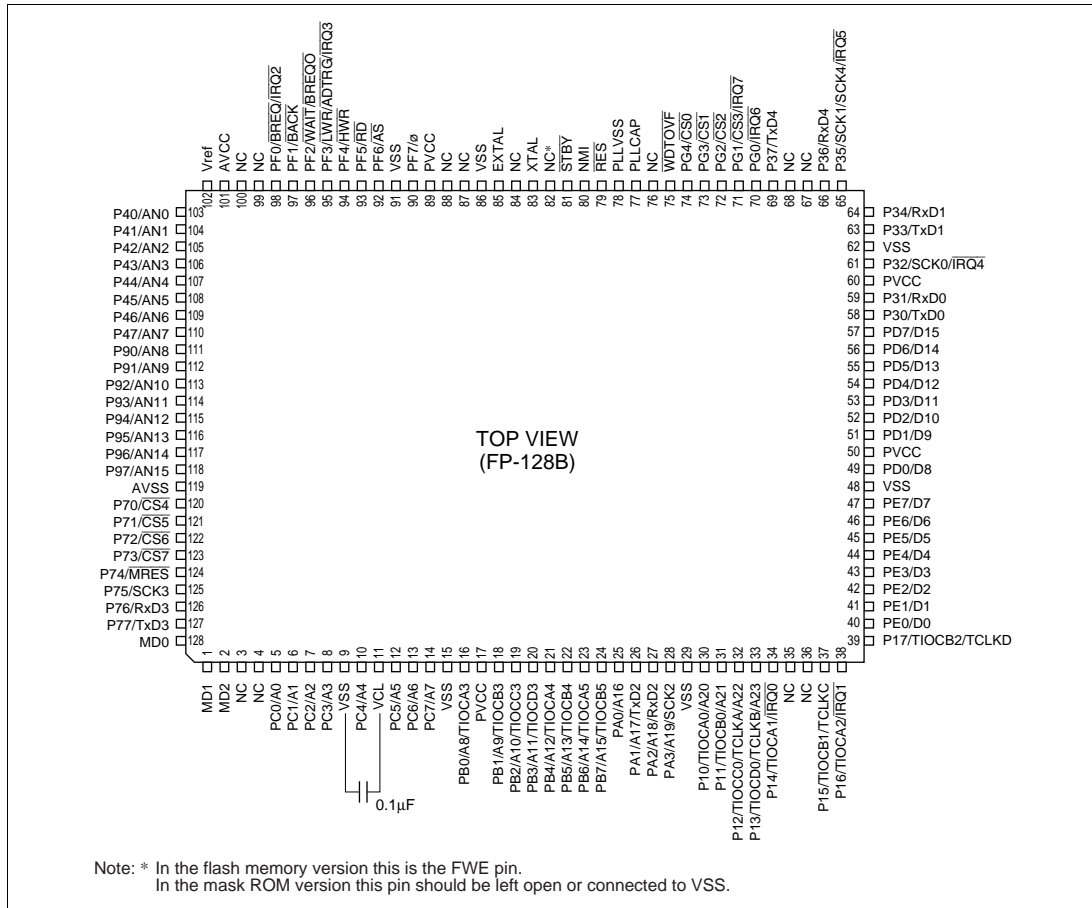
Figure 1-3 (c) H8S/2695 Pin Arrangement (FP-128B: Top View)
