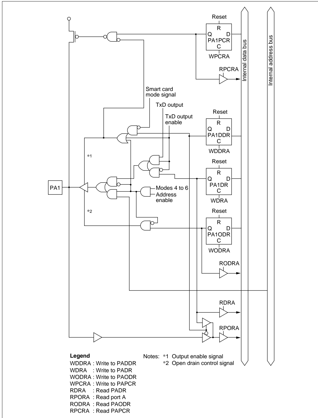
Figure C-6 (b) Port A Block Diagram (Pin PA1)
