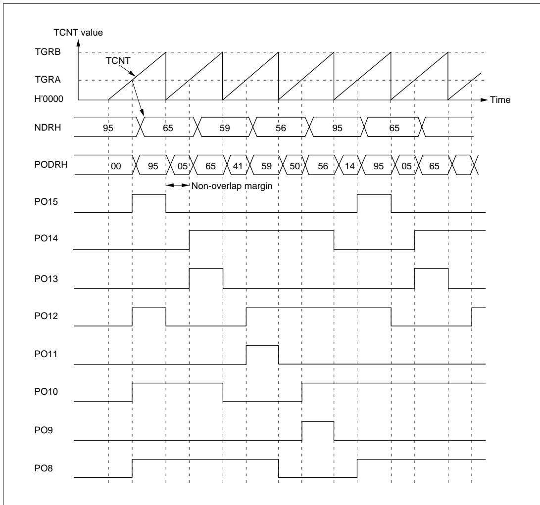
Figure 12-7 Non-Overlapping Pulse Output Example (Four-Phase Complementary)
