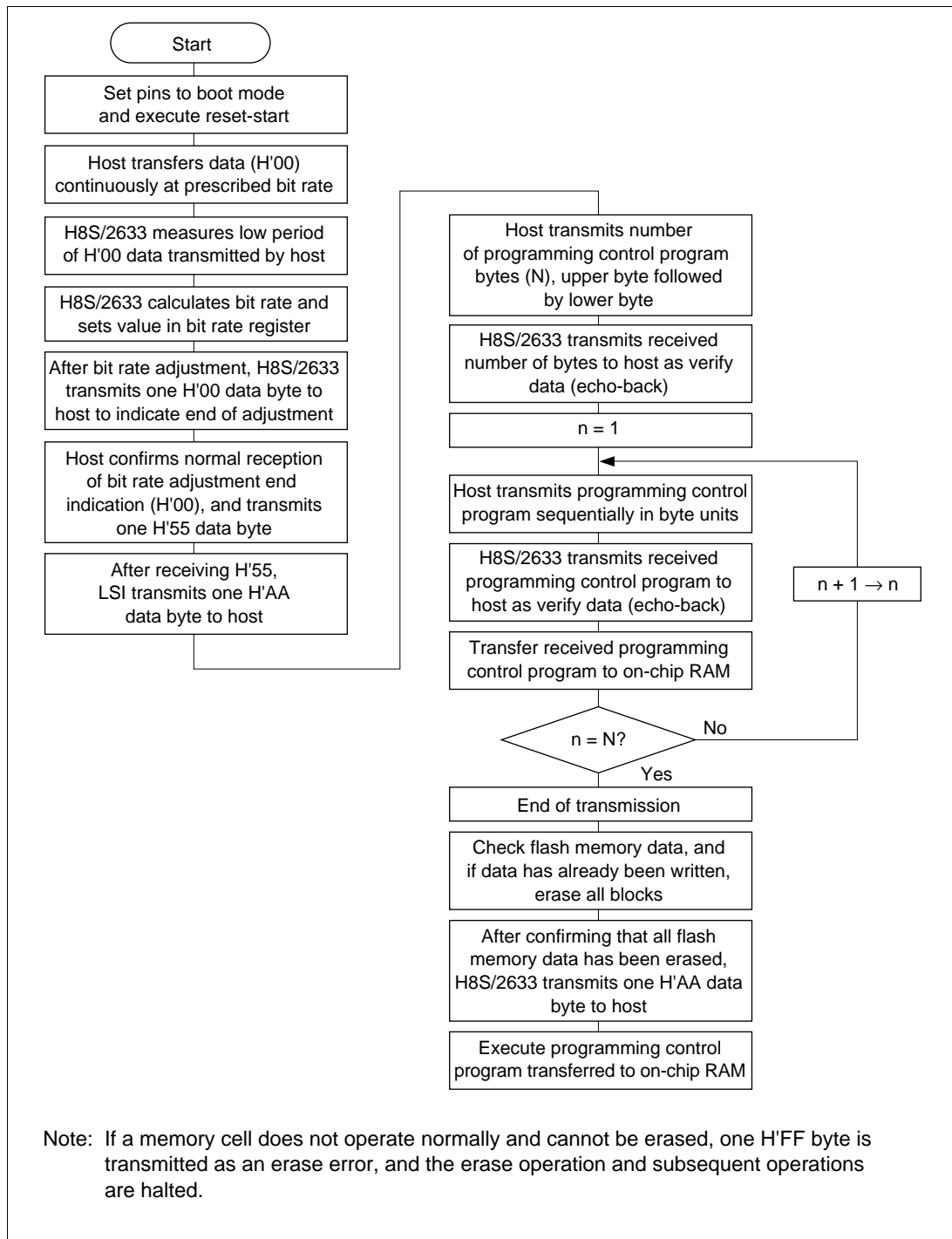
Figure 22-8 Boot Mode Execution Procedure
