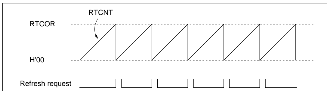
Figure 7-25 RTCNT Operation
