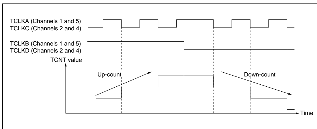
Figure 11-30 Example of Phase Counting Mode 2 Operation
