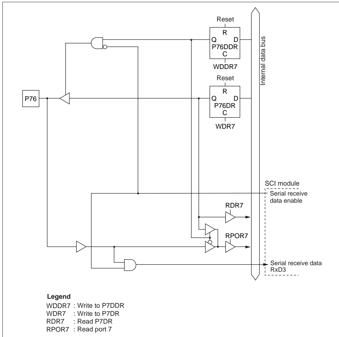
Figure C-16 (f) Port 7 Block Diagram (Pin P76)
