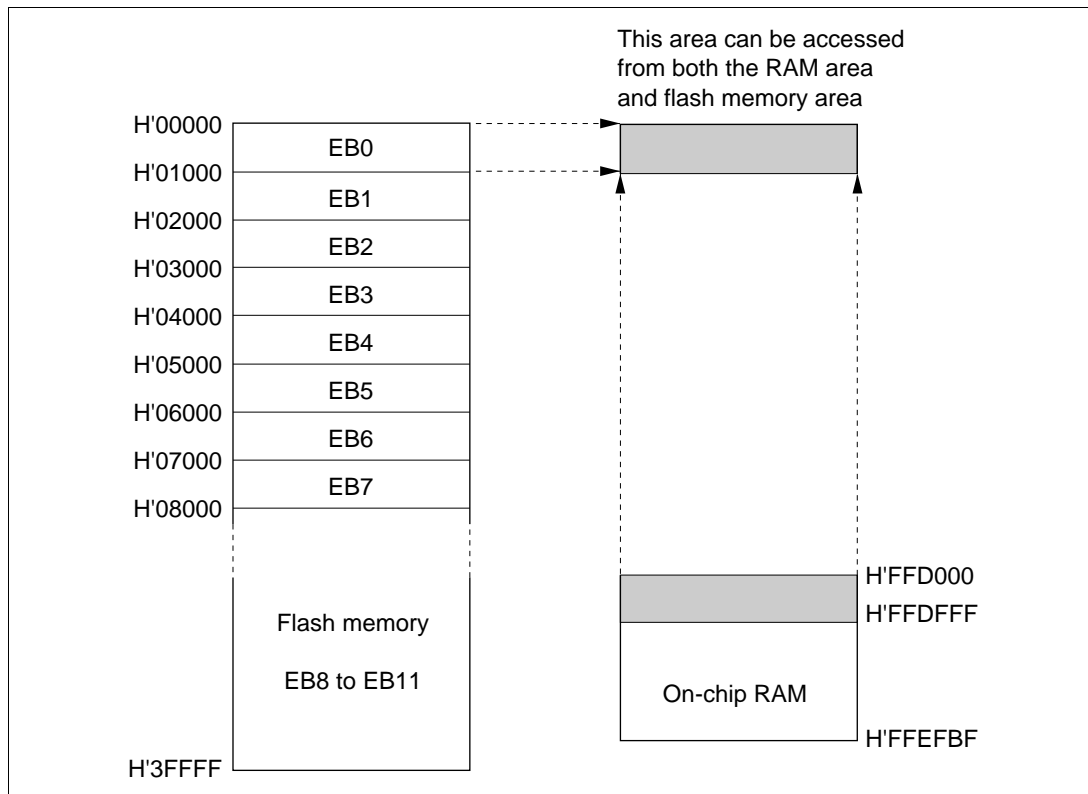
Figure 22-16 Example of RAM Overlap Operation
