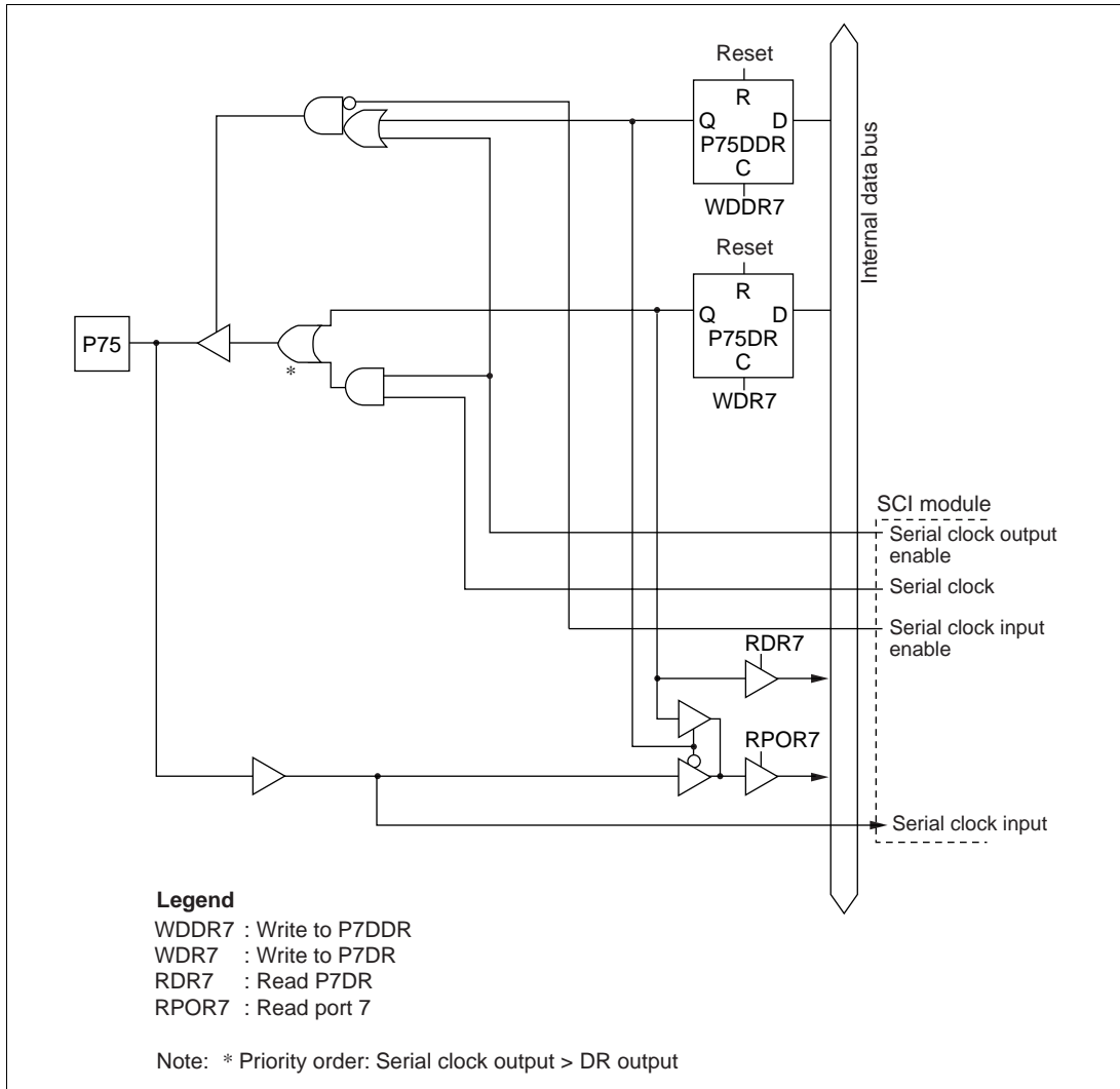
Figure C-16 (e) Port 7 Block Diagram (Pin P75)
