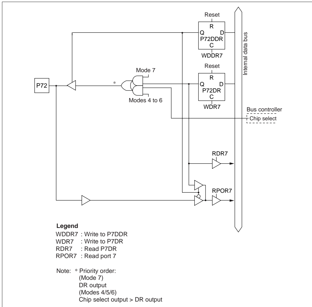
Figure C-16 (b) Port 7 Block Diagram (Pin P72)
