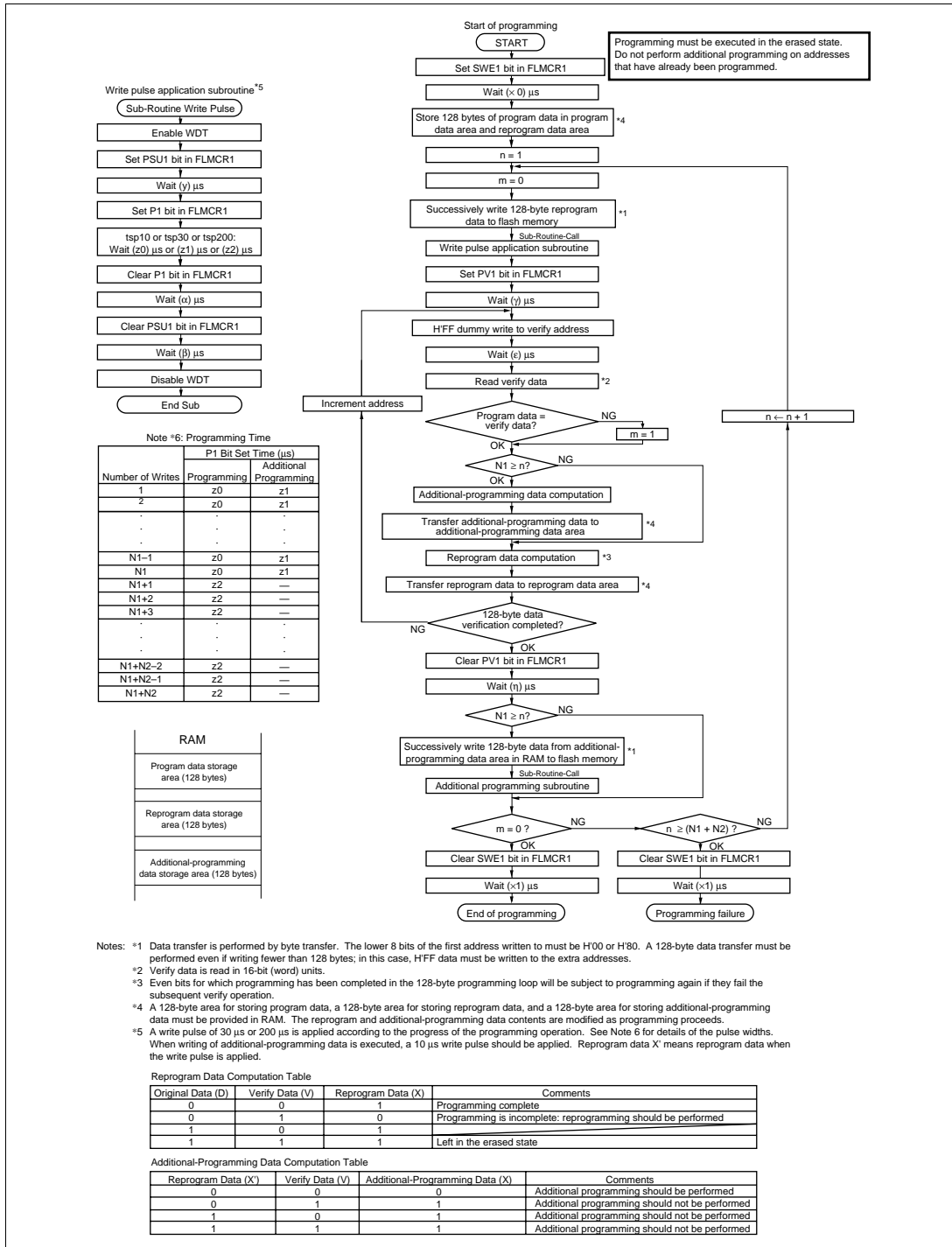
Figure 22-12 Program/Program-Verify Flowchart
