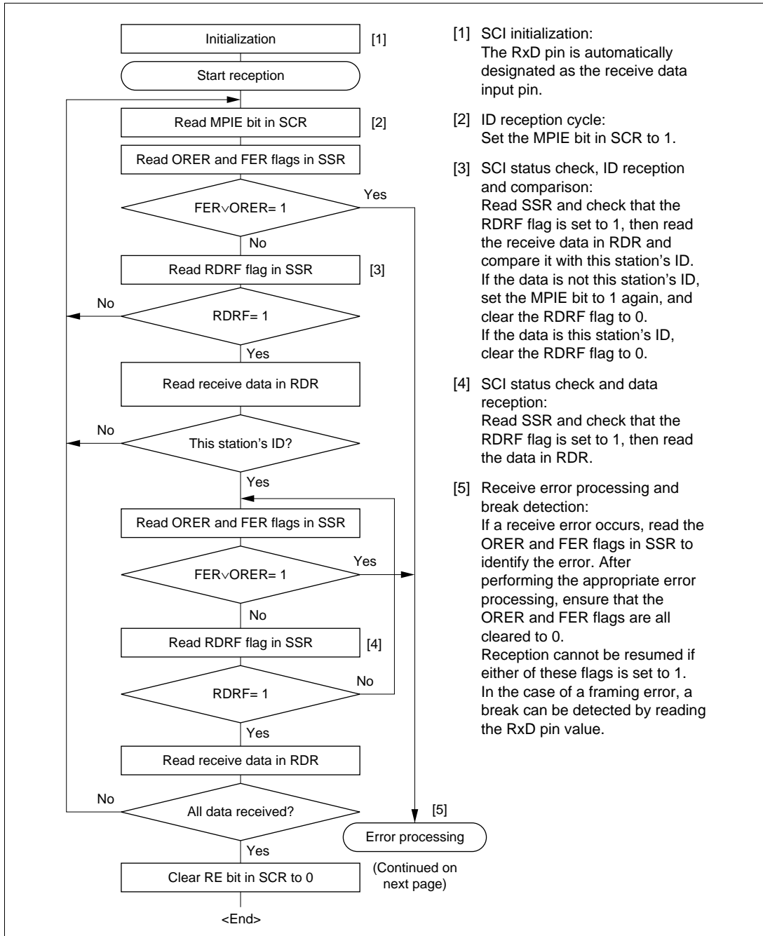
Figure 16-12 Sample Multiprocessor Serial Reception Flowchart
