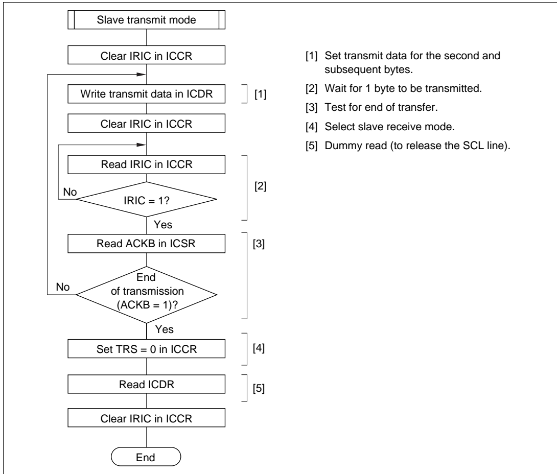
Figure 18-20 Flowchart for Slave Receive Mode (Example)
