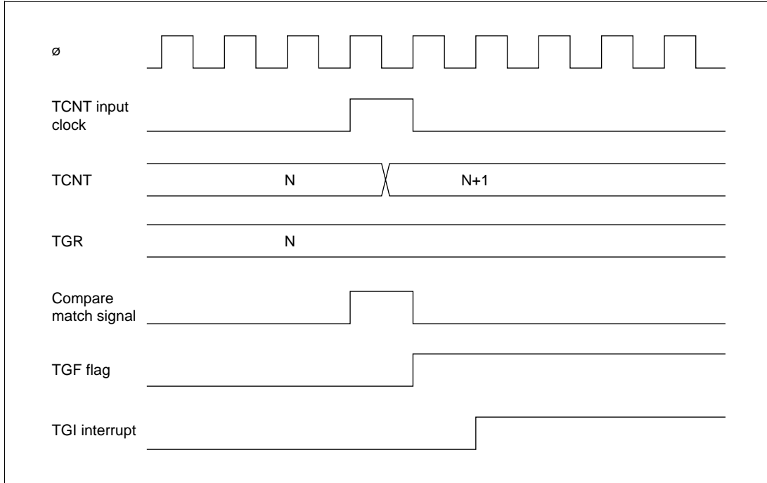
Figure 11-42 TGI Interrupt Timing (Compare Match)
