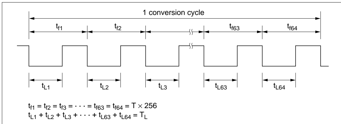
Figure 14-4 (2) Output Waveform
