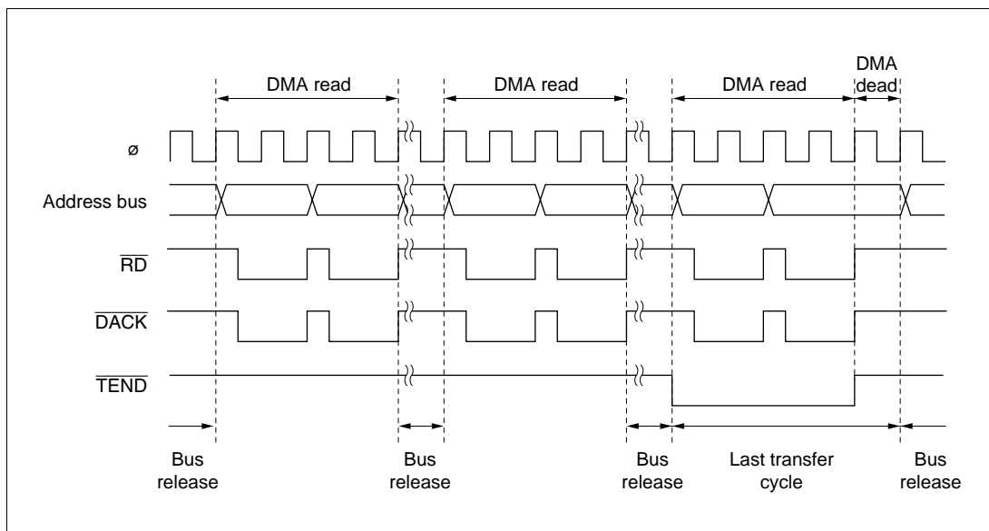
Figure 8-28 Example of Single Address Mode (Word Read) Transfer
