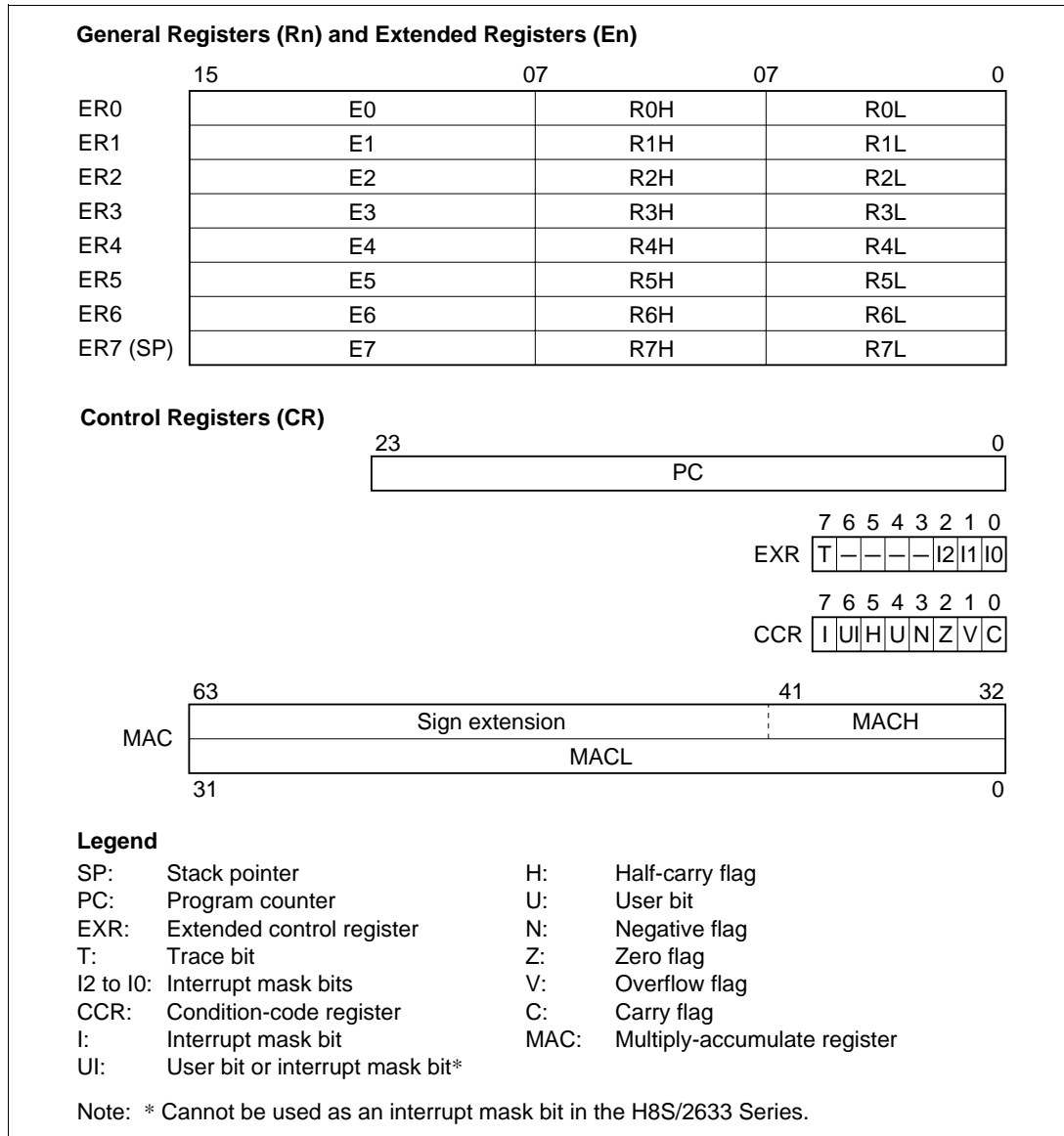
Figure 2-7 CPU Registers
