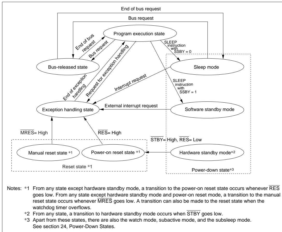
Figure 2-15 State Transitions
