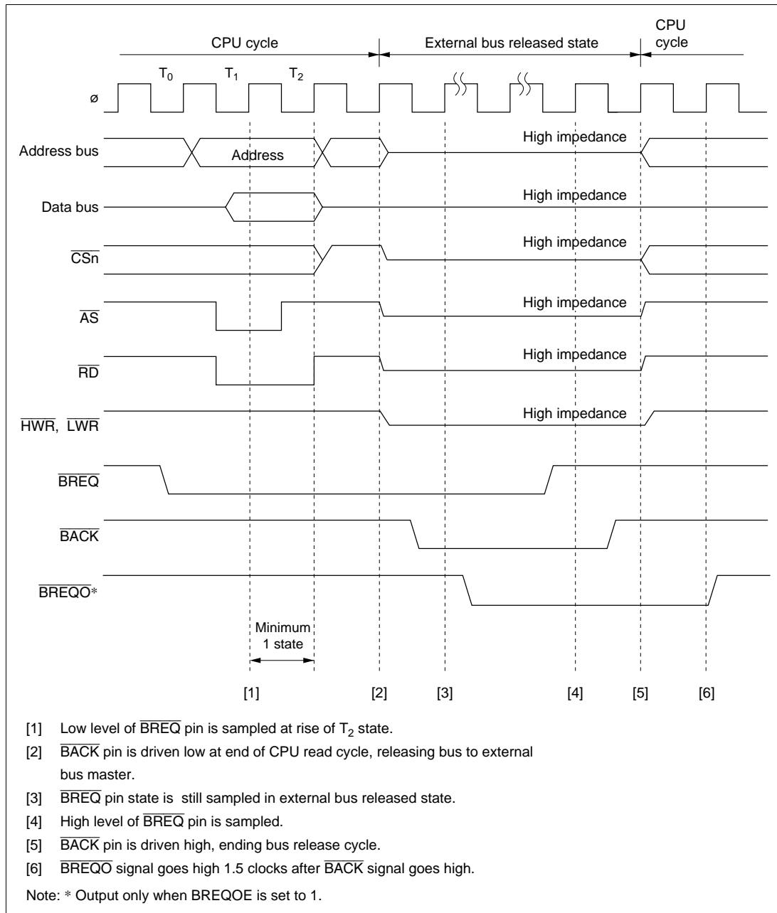
Figure 7-39 Bus-Released State Transition Timing
