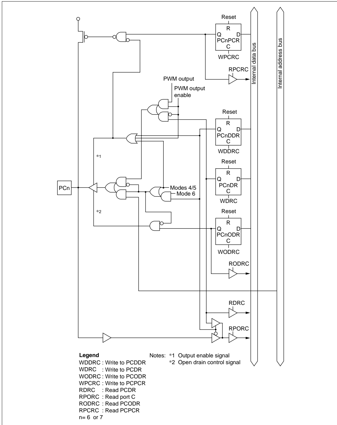
Figure C-8 (b) Port C Block Diagram (Pins PC6 and PC7)
