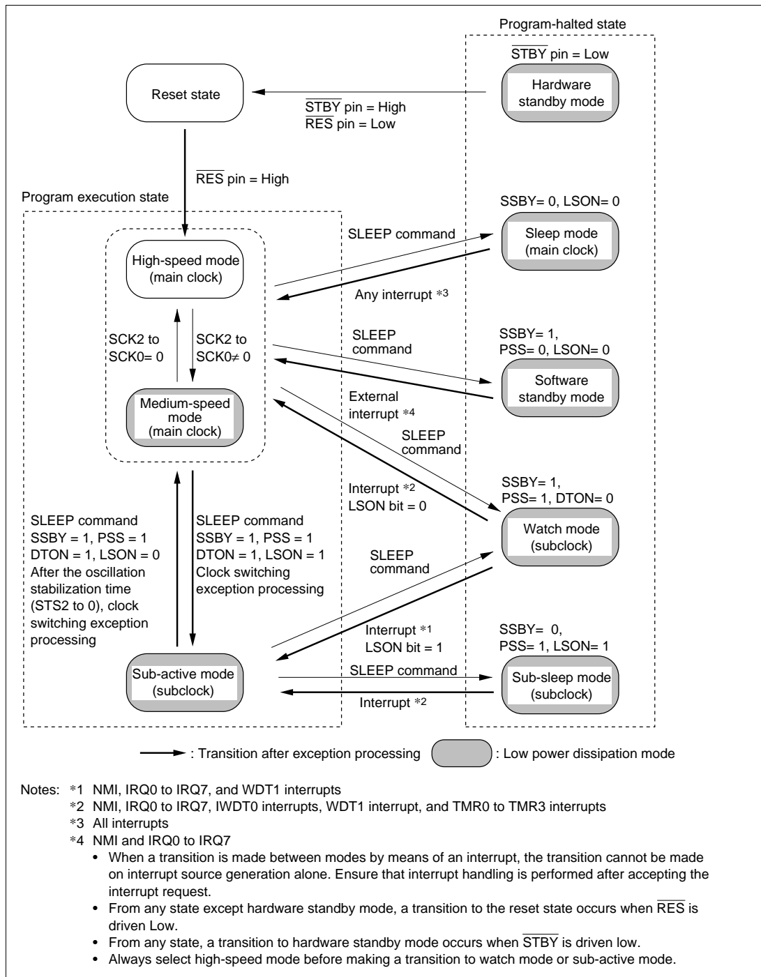
Figure 24-1(a) Mode Transition Diagram (H8S/2633 Series, H8S/2633R)
