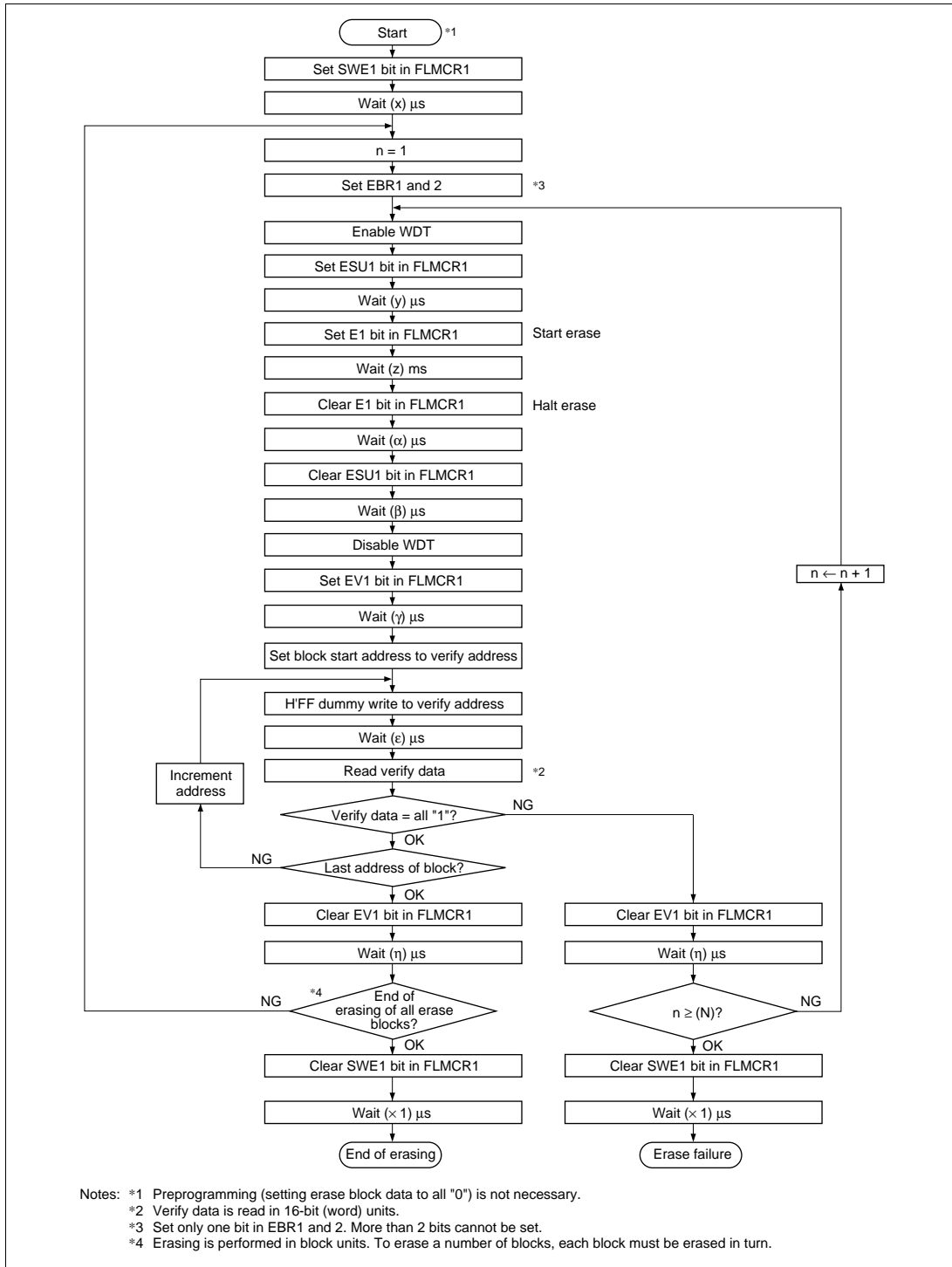
Figure 22-13 Erase/Erase-Verify Flowchart
