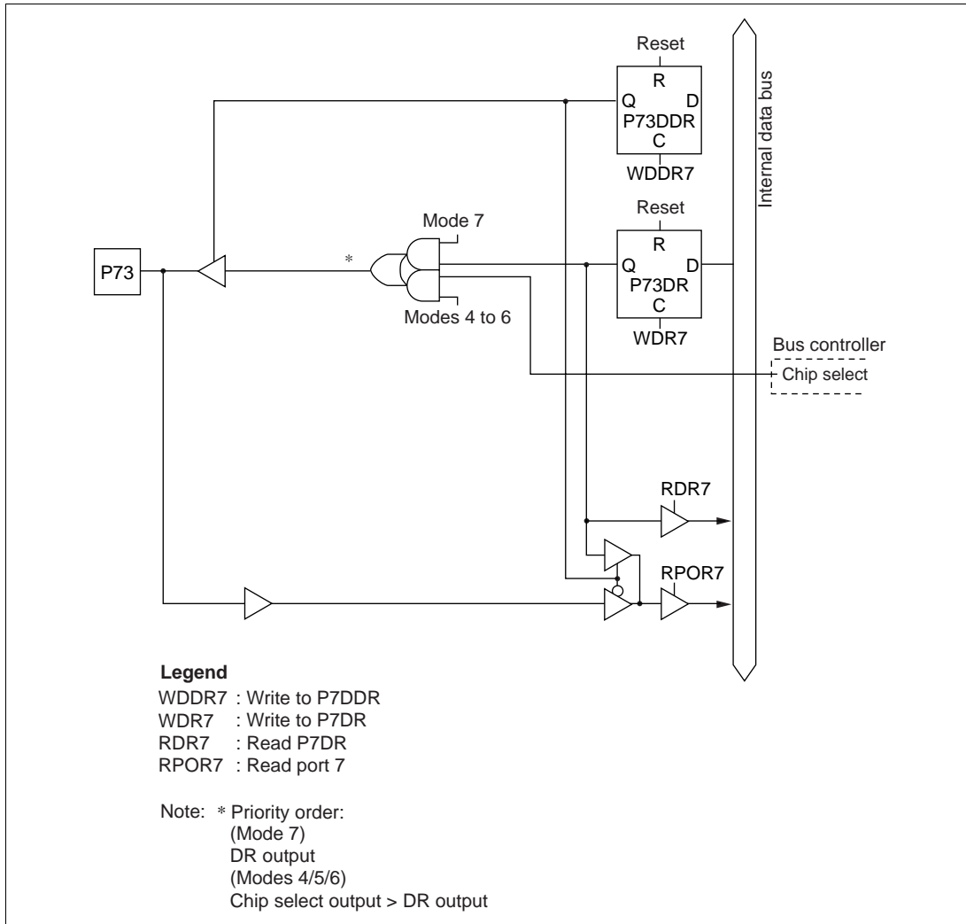
Figure C-16 (c) Port 7 Block Diagram (Pin P73)
