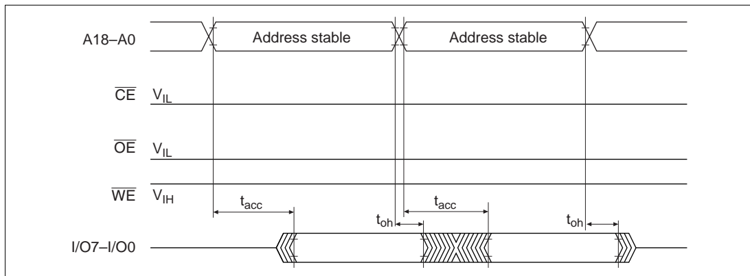
Figure 22-21 \overline{CE} and \overline{OE} Enable State Read Timing Waveforms
