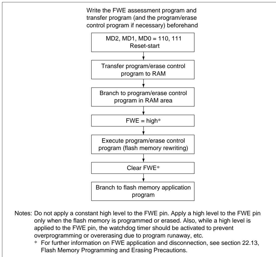
Figure 22-10 User Program Mode Execution Procedure
