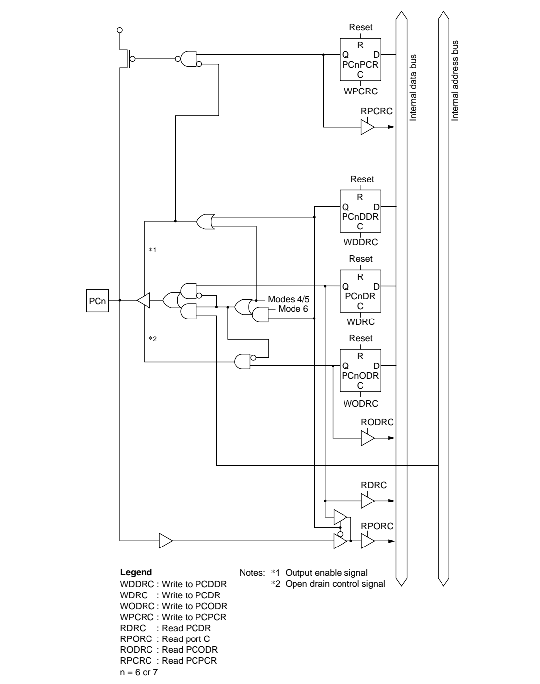
Figure C-20 (b) Port C Block Diagram (Pins PC6 and PC7)
