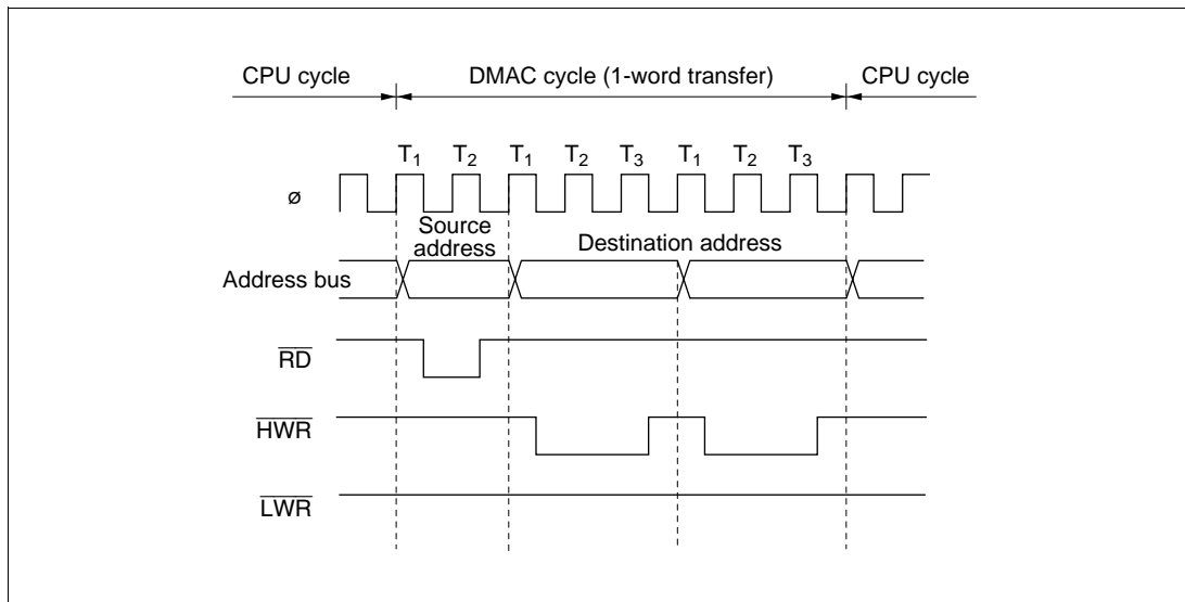
Figure 8-18 Example of DMA Transfer Bus Timing
