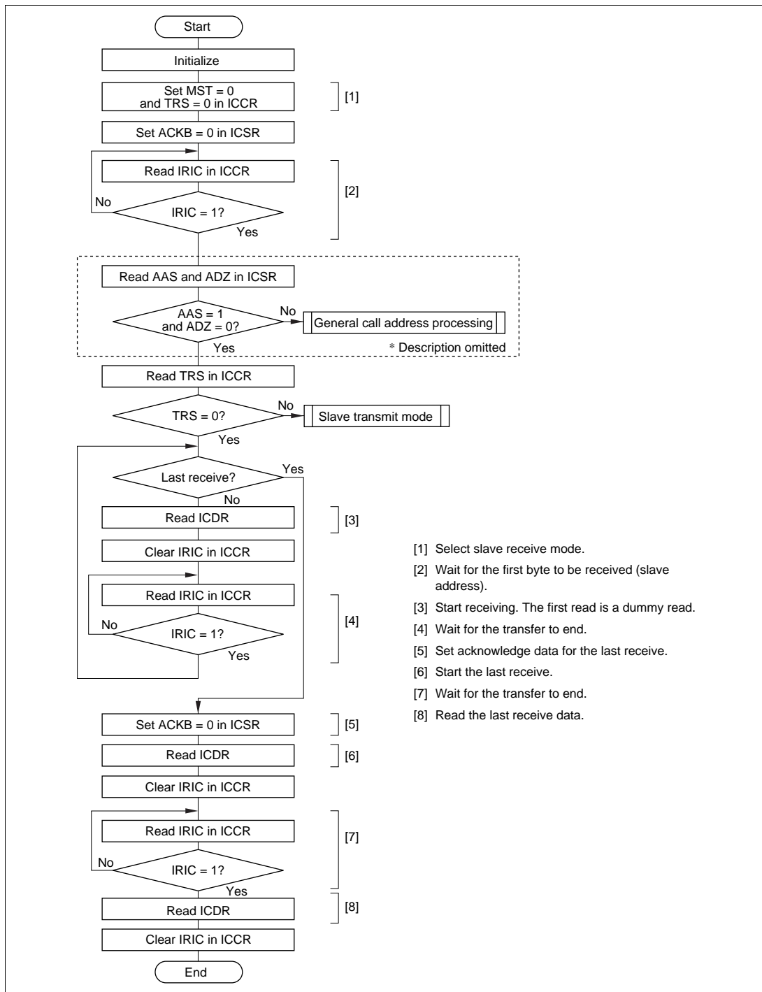
Figure 18-19 Flowchart for Slave Transmit Mode (Example)
