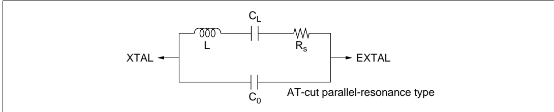
Figure 23B-3 Crystal Resonator Equivalent Circuit
