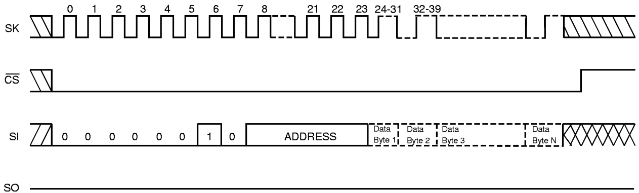
Figure 9. HOLD Timing
