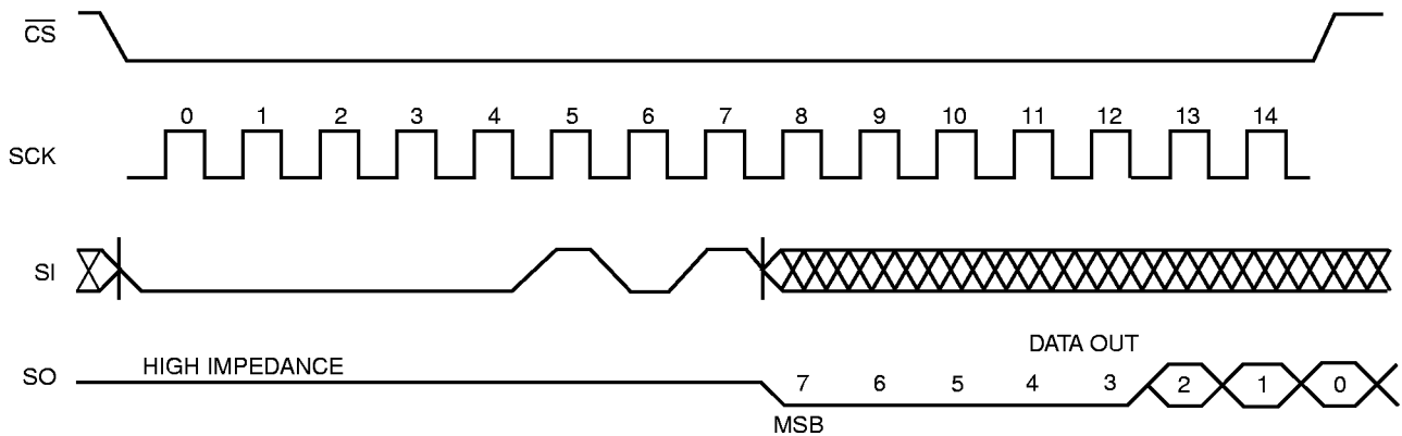
Figure 5. RDSR Timing
