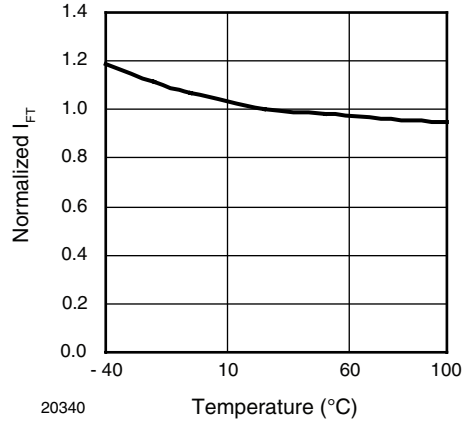
20340 Figure 5. Normalized Trigger Current vs. Temperature
