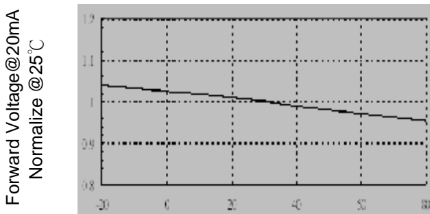
Fig.3 Forward Voltage vs. Temperature
