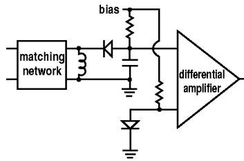
Figure 16. Differential Detector.
