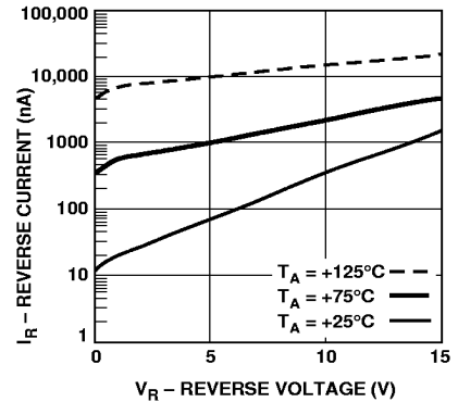
Figure 6. Reverse Current vs. Reverse Voltage at Temperatures—HSMS-282a Series.
