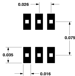
Figure 25. PCB Pad Layout (dimensions in inches).
