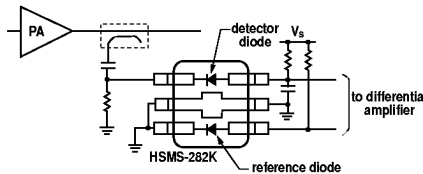
Figure 19. High Isolation Differential Detector.
