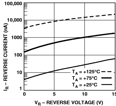
Figure 5. Reverse Current vs. Reverse Voltage at Temperatures—HSMS-281a Series.
