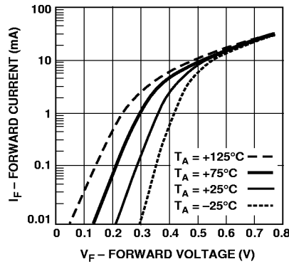
Figure 2. Forward Current vs. Forward Voltage at Temperatures—HSMS-281a Series.
