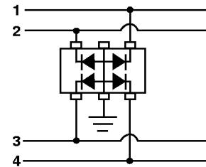
Figure 14. Clamping Four Lines.
