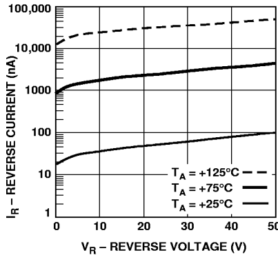
Figure 4. Reverse Current vs. Reverse Voltage at Temperatures—HSMS-280a Series.
