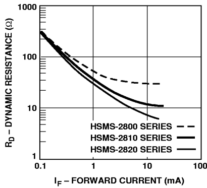
Figure 7. Dynamic Resistance vs. Forward Current.
