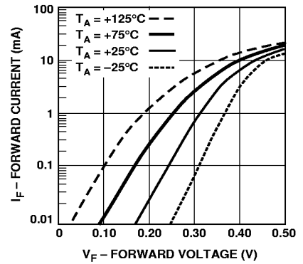
Figure 3. Forward Current vs. Forward Voltage at Temperatures—HSMS-282a Series.
