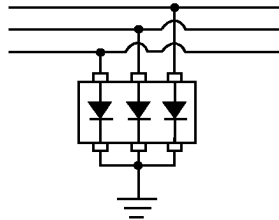
Figure 12. Clamping Three Lines.
