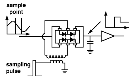
Figure 15. Sampling Circuit.
