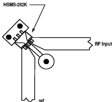
Figure 20. Diode Mounting, HSMS-282K.
