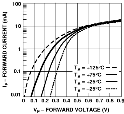
Figure 1. Forward Current vs. Forward Voltage at Temperatures—HSMS-280a Series.
