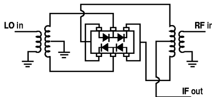
Figure 23. Double Balanced Mixer.
