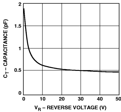
Figure 8. Total Capacitance vs. Reverse Voltage—HSMS-280a Series.
