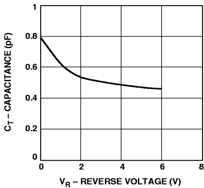
Figure 10. Total Capacitance vs. Reverse Voltage—HSMS-282a Series.
