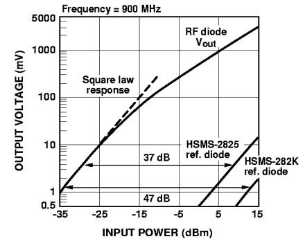
Figure 21. Comparing HSMS-282K with HSMS-2825.
