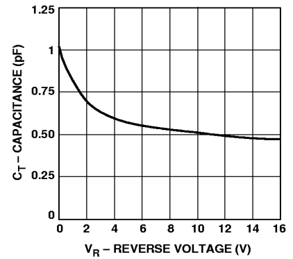
Figure 9. Total Capacitance vs. Reverse Voltage—HSMS-281a Series.
