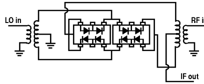
Figure 24. Low Distortion Mixer.
