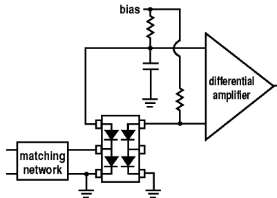
Figure 22. Differential Voltage Doubler, HSMS-282P.
