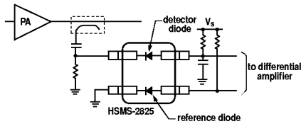
Figure 17. Conventional Differential Detector.
