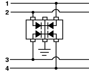
Figure 13. Clamping Four Lines.
