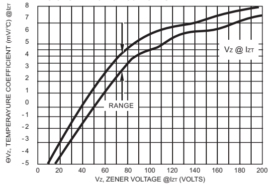
FIG.5- UNIT 10 TO 200 VOLTS
