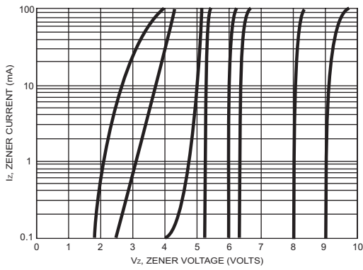
FIG.8- VZ = 3.9 THRU 10 VOLTS
