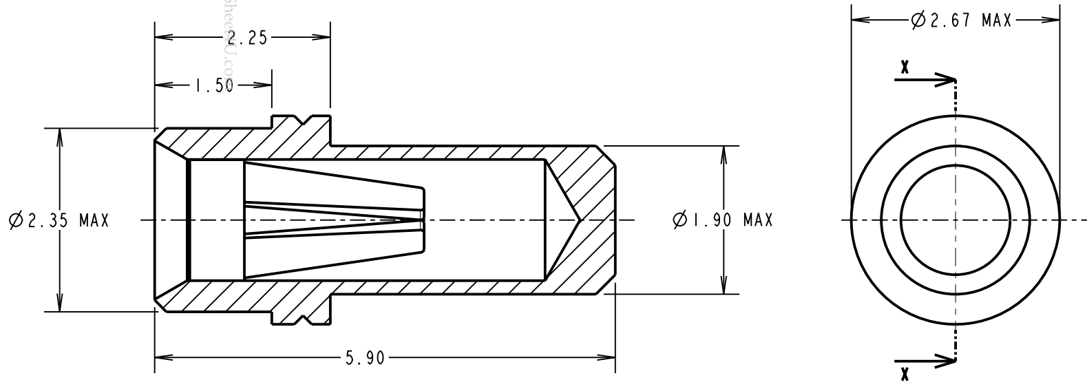
SECTION X-X
