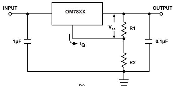
Circuit For Increasing Output Voltage
