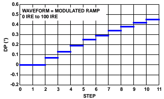
FIGURE 12. DIFFERENTIAL PHASE
