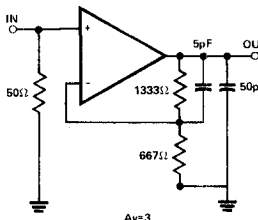
SLEW RATE AND TRANSIENT RESPONSE
