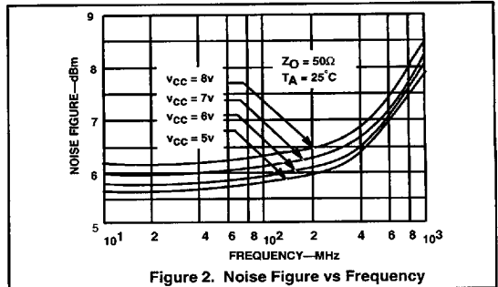
Figure 2. Noise Figure vs Frequency
