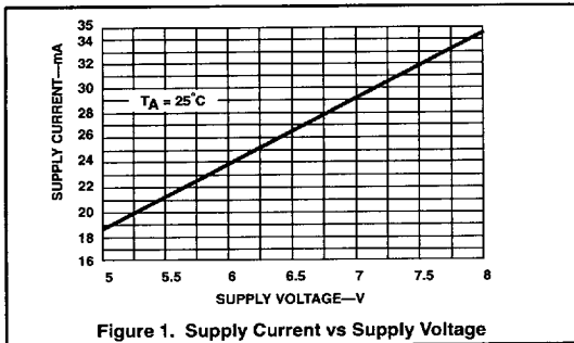
Figure 1. Supply Current vs Supply Voltage
