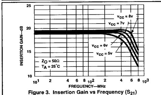
Figure 3. Insertion Gain vs Frequency (S 21 )
