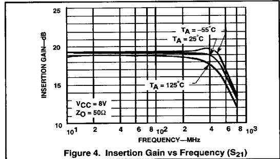
Figure 4. Insertion Gain vs Frequency (S 21 )
