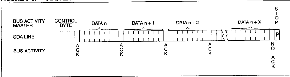
FIGURE 9-3: SEQUENTIAL READ
