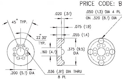
615-075 8 LEADS
