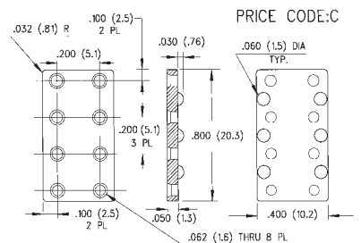
408-080
