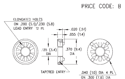
607-075 12 LEADS
