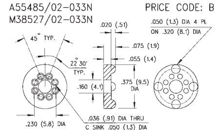
617-075 8 LEADS
