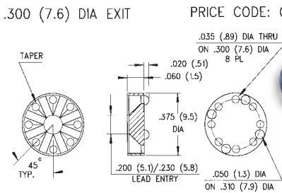
711-085 8 LEADS
