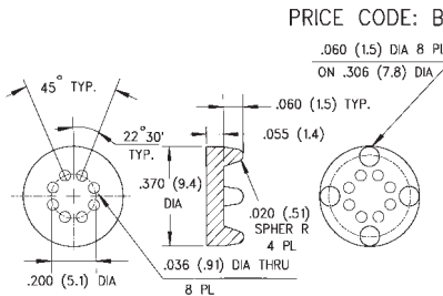
603-115 8 LEADS
