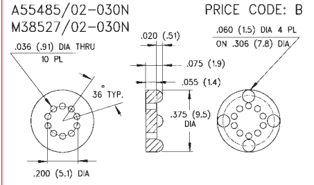
611-075 10 LEADS
