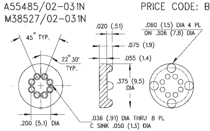
610-075 8 LEADS
