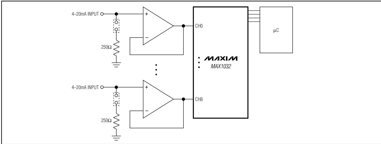
Figure 19. 4-20mA Application
