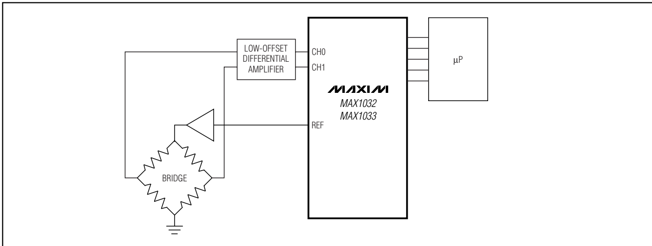
Figure 20. Bridge Application
