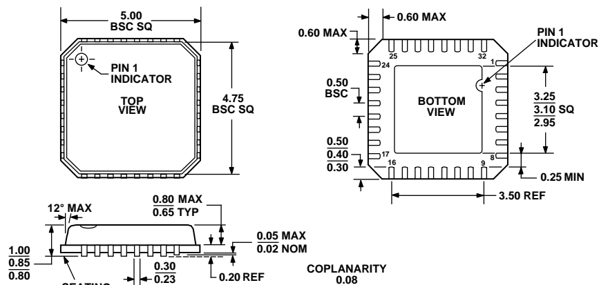
Figure 46. 32-Lead Lead Frame Chip Scale Package [LFCSP] (CP-32-2)
