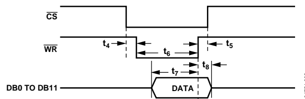
Figure 37. AD7938-6 Parallel Interface—Write Cycle Timing for Word Mode Operation ( \overline{W/B} = 1 )
