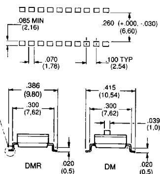
Printed circuit board layout
