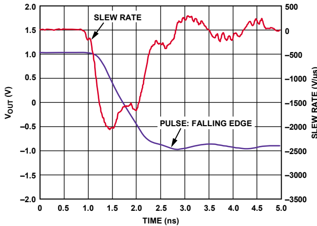
Figure 20. ADV3226 Falling Edge Slew Rate
