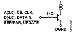
Figure 61. Logic Input
