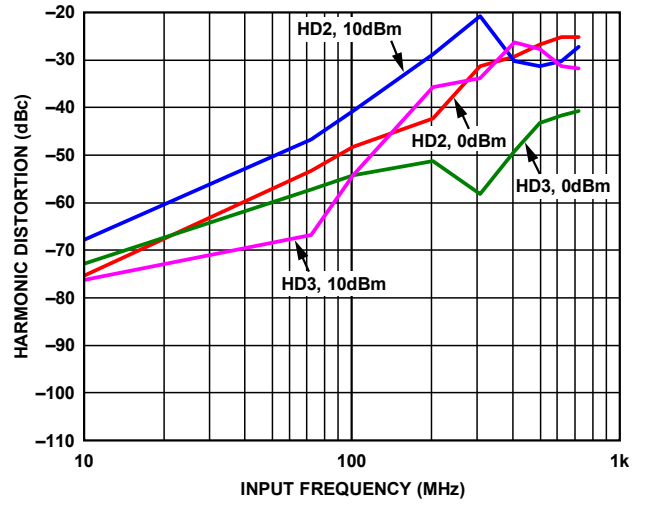
Figure 57. ADV3227 Harmonic Distortion (Input Referred), 100 Ω Load
