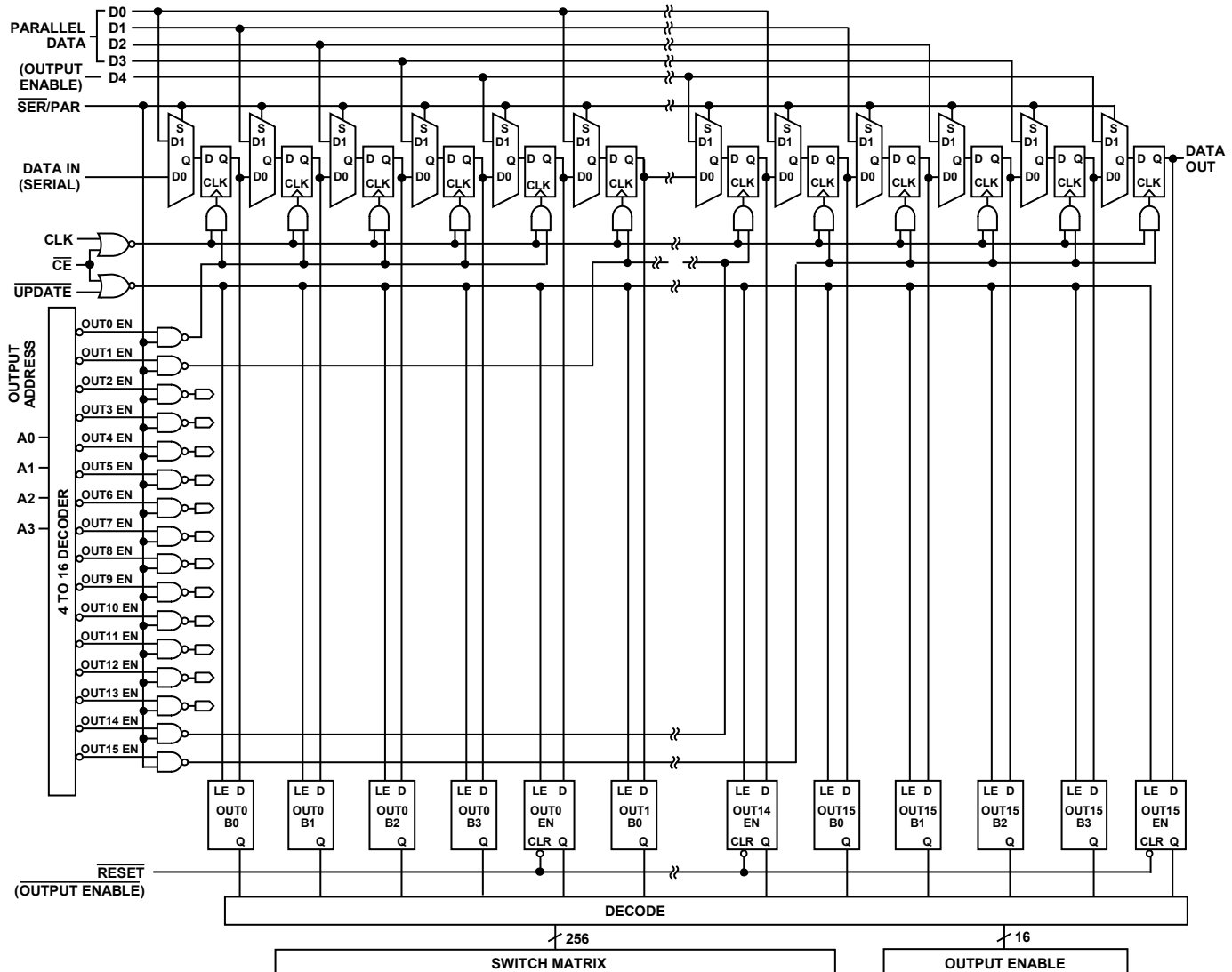
Figure 6. Logic Diagram
