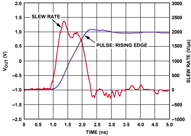
Figure 19. ADV3226 Rising Edge Slew Rate
