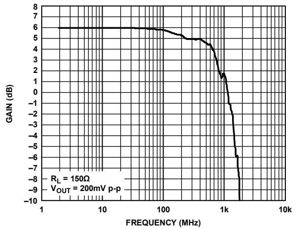
Figure 10. ADV3227 Small Signal Frequency Response
