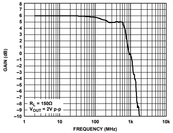
Figure 11. ADV3227 Large Signal Frequency Response
