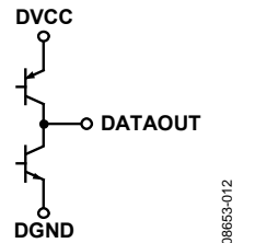
Figure 64. Logic Output
