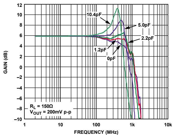
Figure 12. ADV3227 Small Signal Frequency Response, R_L = 150\Omega
