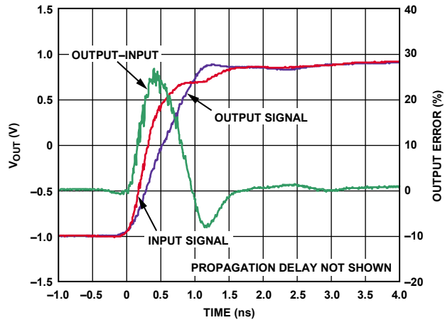
Figure 21. ADV3226 Settling Time
