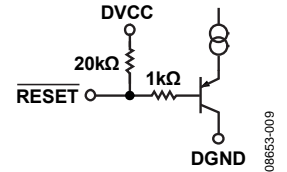
Figure 63. Reset Input
