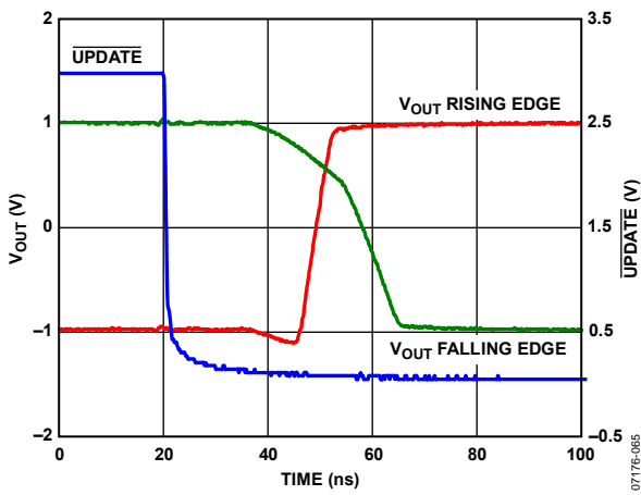
Figure 36. ADV3200 Switching Time
