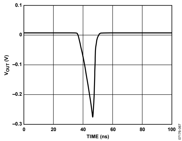
Figure 39. ADV3200 Switching Glitch
