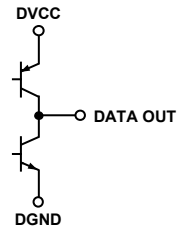
Figure 13. Logic Output (See Also Figure 16)
