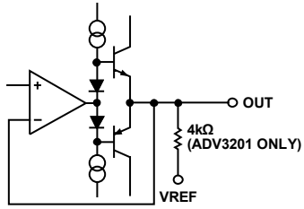
Figure 7. Enabled Output (See Also Figure 16)
