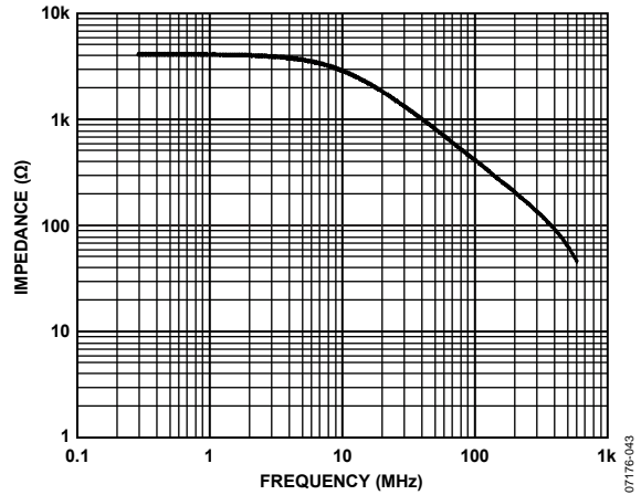
Figure 71. ADV3201 Output Impedance, Disabled
