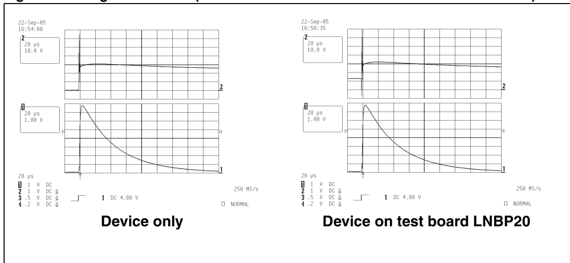
Figure 6. Surge tests +4 kV (Standard IEC61000-4-5 - with series resistor of 12 \Omega )
