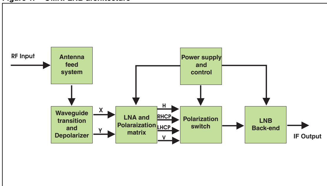
Figure 1. OMNI-LNB architecture
