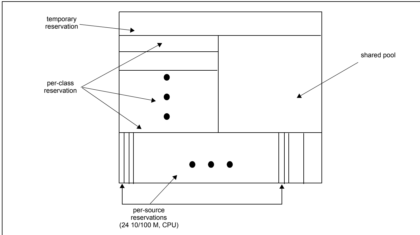
Figure 10 - Buffer Partition Scheme Used to Implement MVTX2602 Buffer Management
