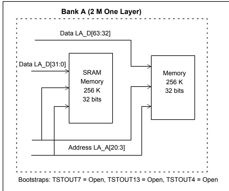
Figure 9 - Memory Configuration for 1 Bank, 1 Layer, 2 MB
