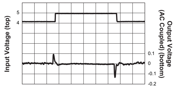
Line Transient
