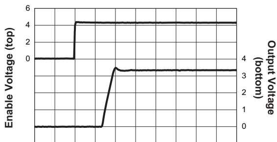
Soft-Start
