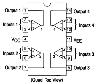
P SUFFIX PLASTIC PACKAGE CASE 646
