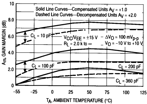
Figure 22. Gain Margin versus Temperature
