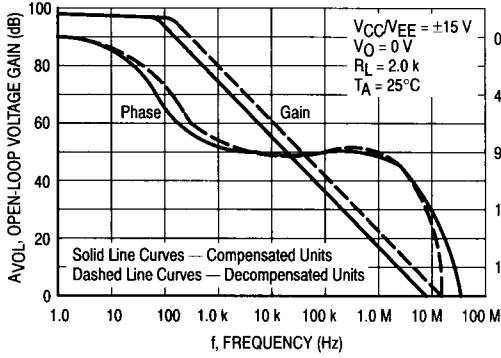
Figure 14. Open-Loop Voltage Gain and Phase versus Frequency
