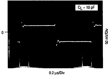
Figure 24. Small-Signal
