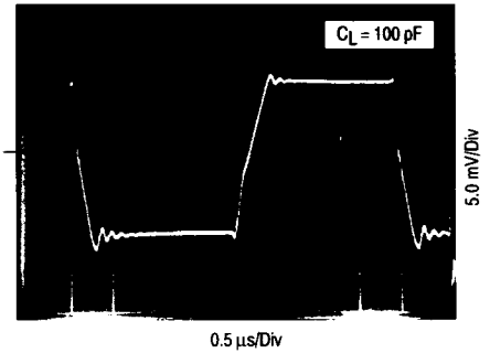
Figure 27. Large-Signal
