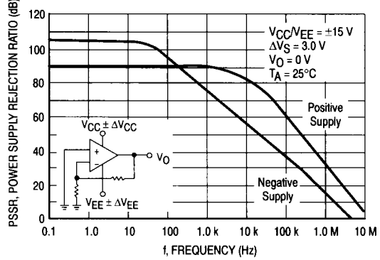
Figure 29. Power Supply Rejection Ratio versus Frequency
