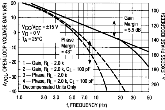
Figure 16. Open-Loop Voltage Gain and Phase versus Frequency
