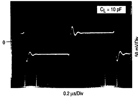
Figure 26. Small-Signal
