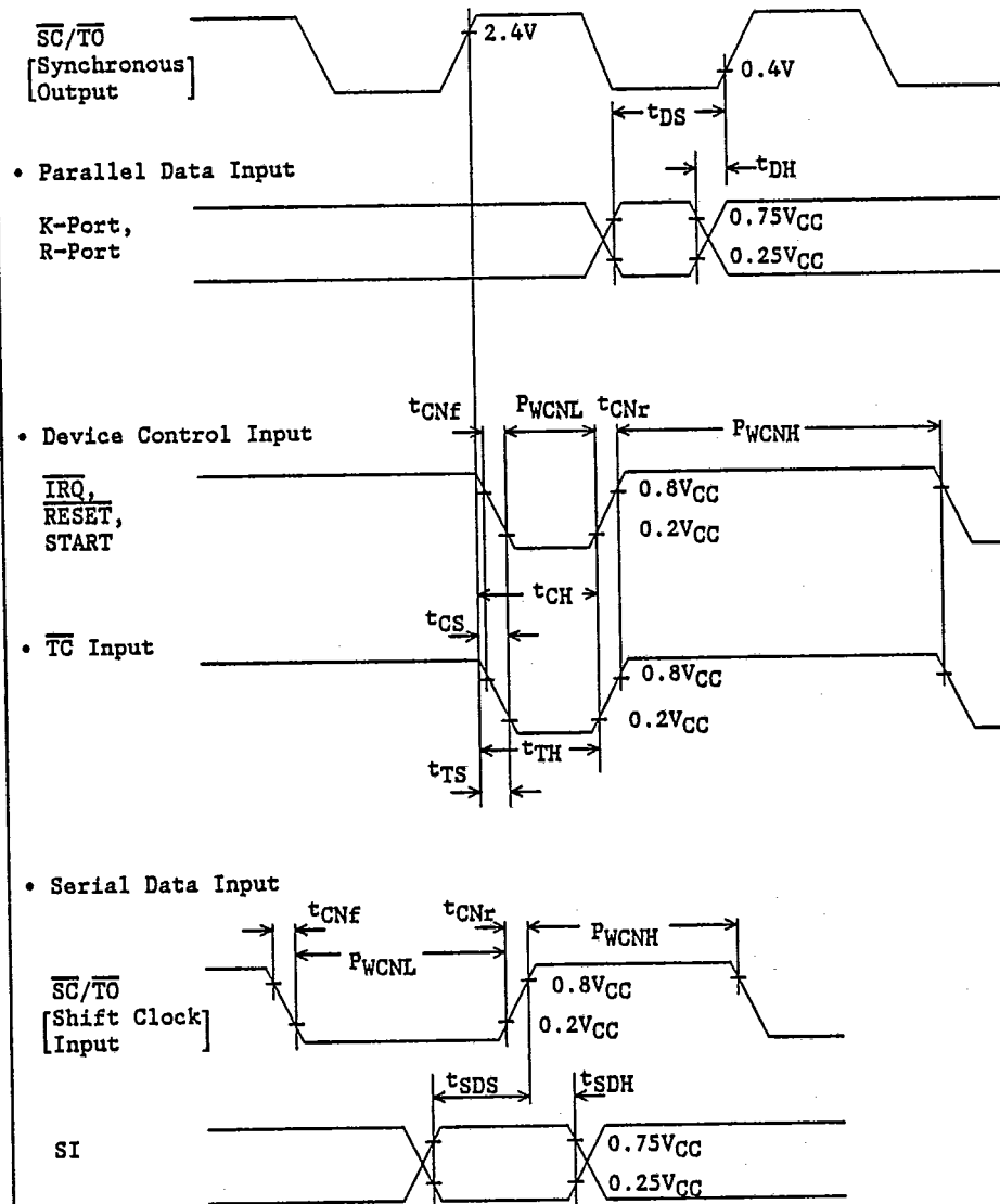
Fig. 11: INPUT TIMING
