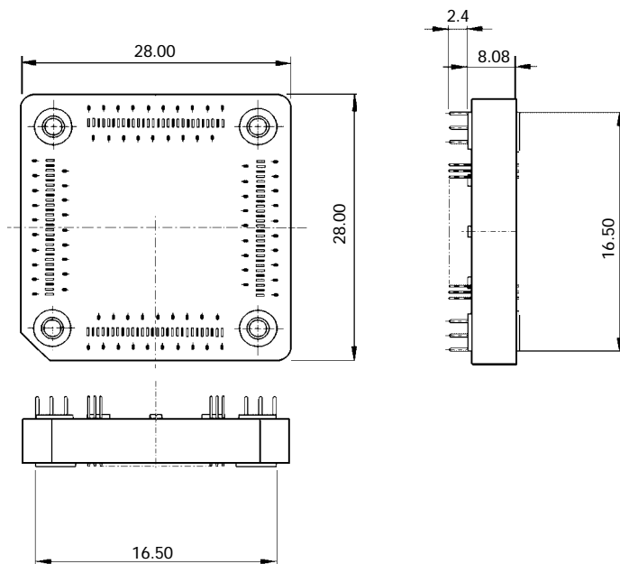
Adapter PCB-Layout (IC149-120-*43-B5)
