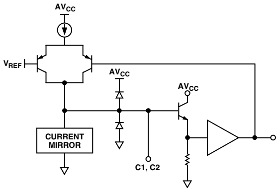
Figure 4. Compensation Pin, C1 or C2
