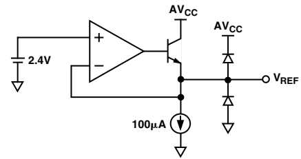
Figure 6. 2.4 V Reference
