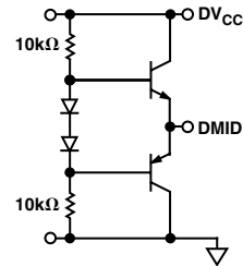
Figure 7. DMID Reference
