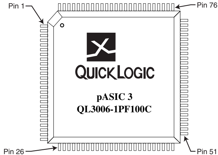
Figure 9: Top View of 100 Pin TQFP
