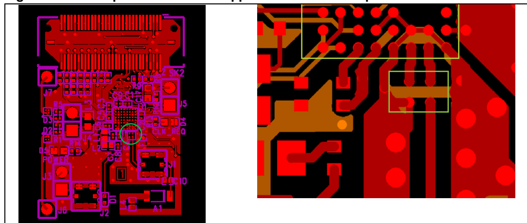
Figure 10. Example of transceiver application board land pattern
