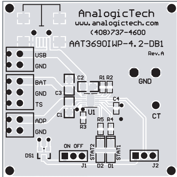
Figure 4: AAT3690 Evaluation Board Top Side Layout.
