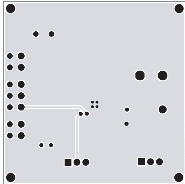
Figure 5: AAT3690 Evaluation Board Bottom Side Layout.
