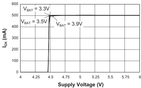
USB Fast Charge Current vs. Supply Voltage ( R_{USBSET}; USB = 8.06k\Omega )
