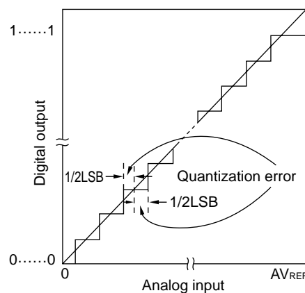
Figure 13-13. Quantization Error
