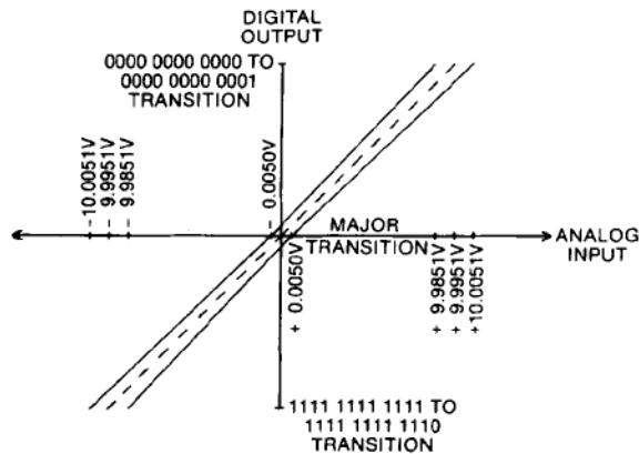
MN5202 ABSOLUTE ACCURACY +25^\circ\text{C}
