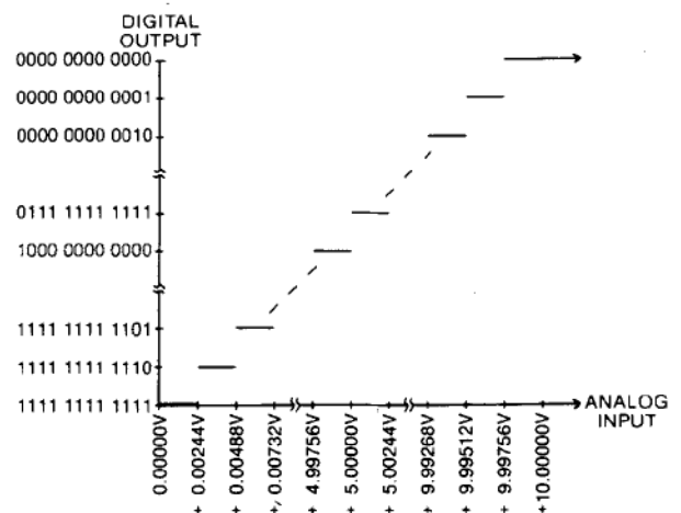
MN5206 TRANSFER FUNCTION
