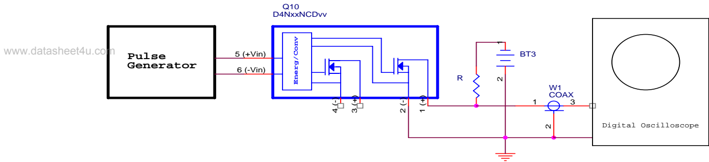
Figure 1 A hook-up setting for performing test of a normal-opened (N.O.) pair
