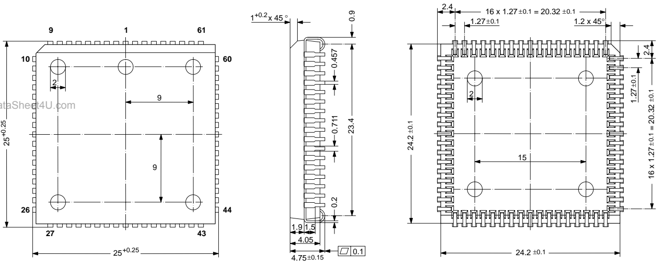
Fig. 3-2: 68-Pin Plastic Leaded Chip Carrier Package (PLCC68) Weight approximately 4.8 g Dimensions in mm
