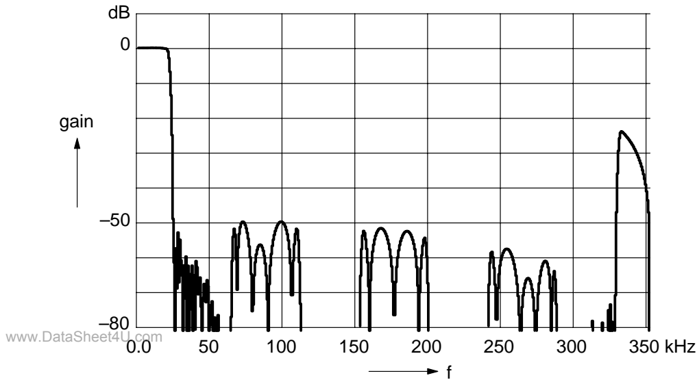
Fig. 2-11: Digital interpolation filter, attenuation
