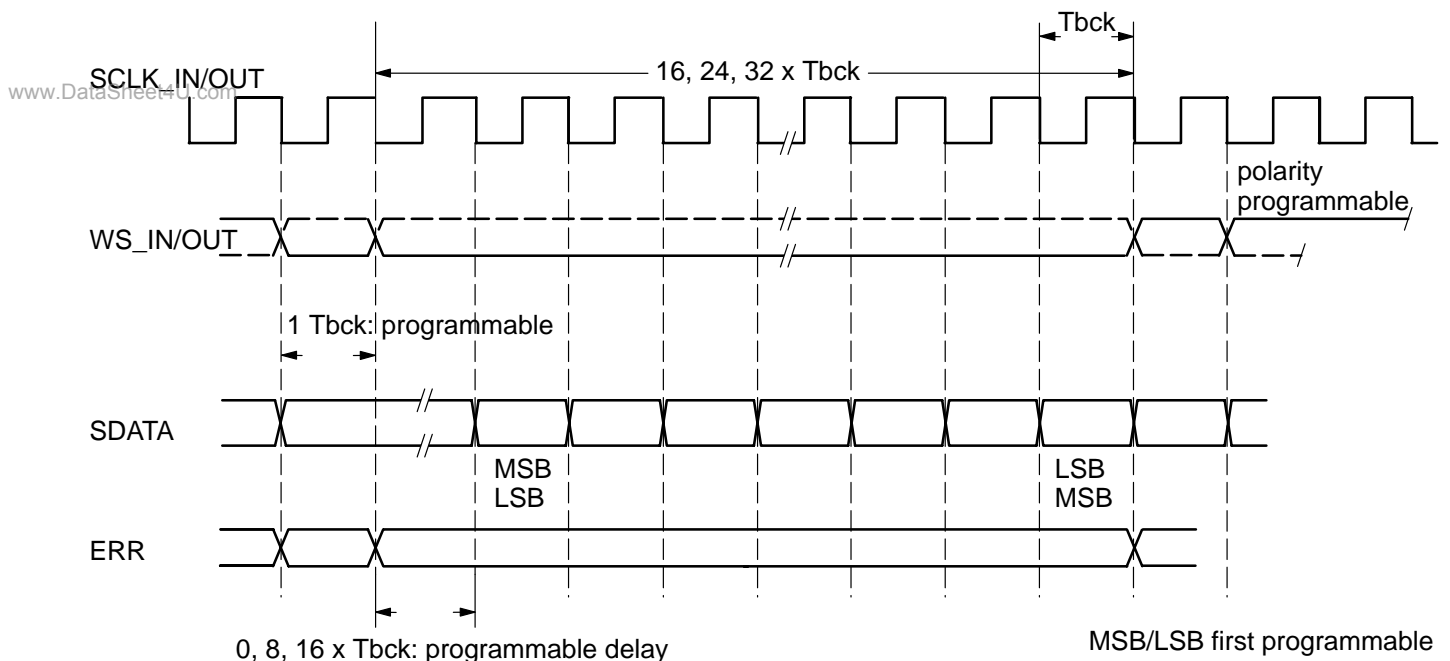
Fig. 2-13: Timing of the signals
