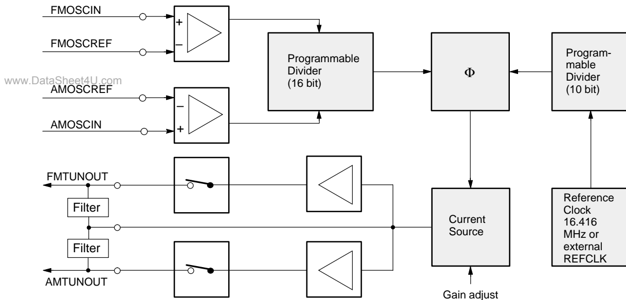
Fig. 5–1: Synthesizer block diagram
