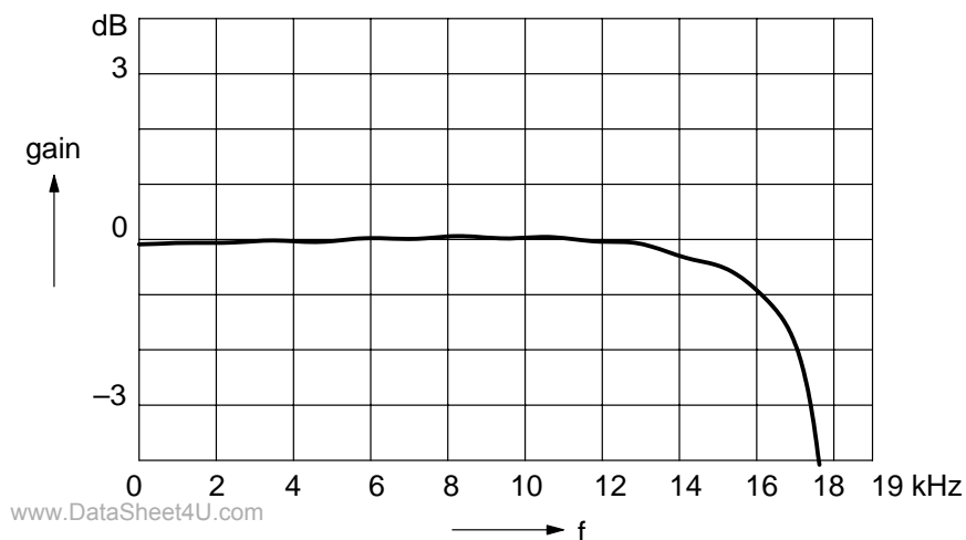
Fig. 2-8: Overall MPX response sum channel
