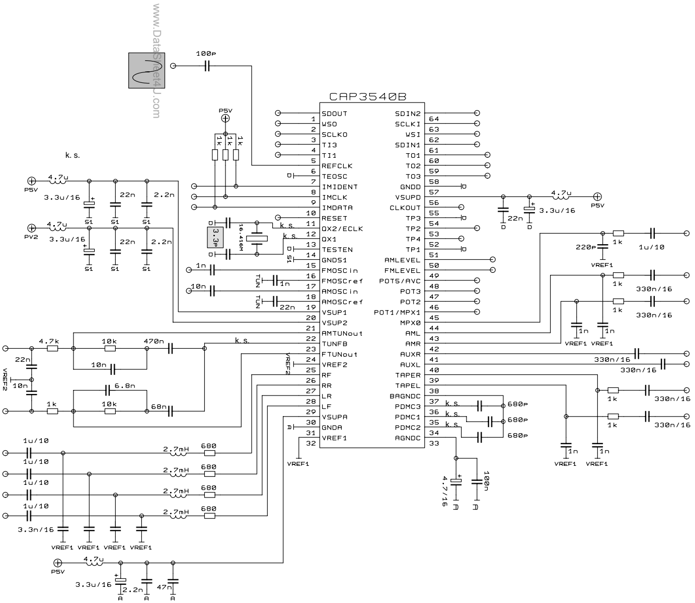
Fig. 7-1: Typical Application Circuit
