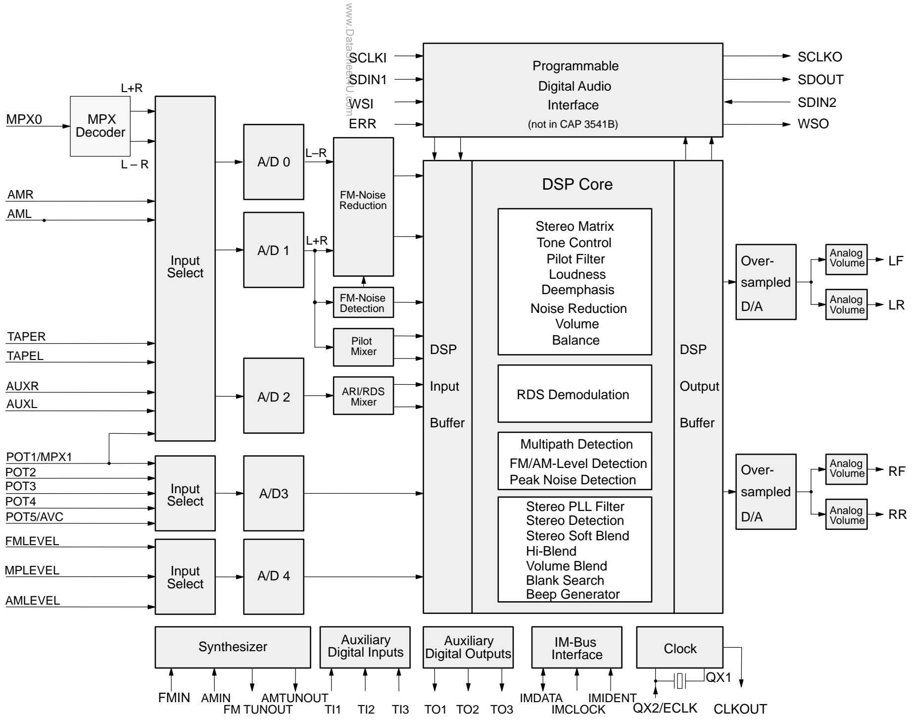
Fig. 2-1: CAP 3540B block diagram
