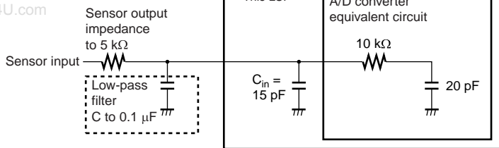
Figure 14.6 Analog Input Circuit Example
