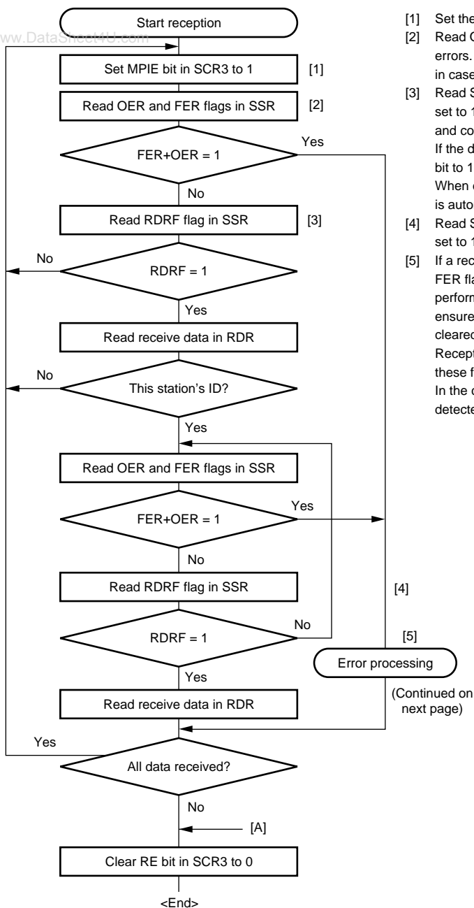
Figure 13.17 Sample Multiprocessor Serial Reception Flowchart (1)
