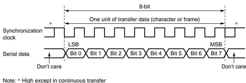
Figure 13.9 Data Format in Clocked Synchronous Communication
