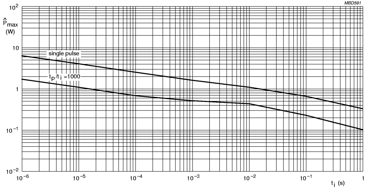
Fig. 10 Pulse on a regular basis for type: RC21 ; maximum permissible peak pulse power ( \hat{P}_{max} ) as a function of pulse duration for R \leq 10 \text{ k}\Omega , single pulse and repetitive pulse t_p/t_i = 1000 .
